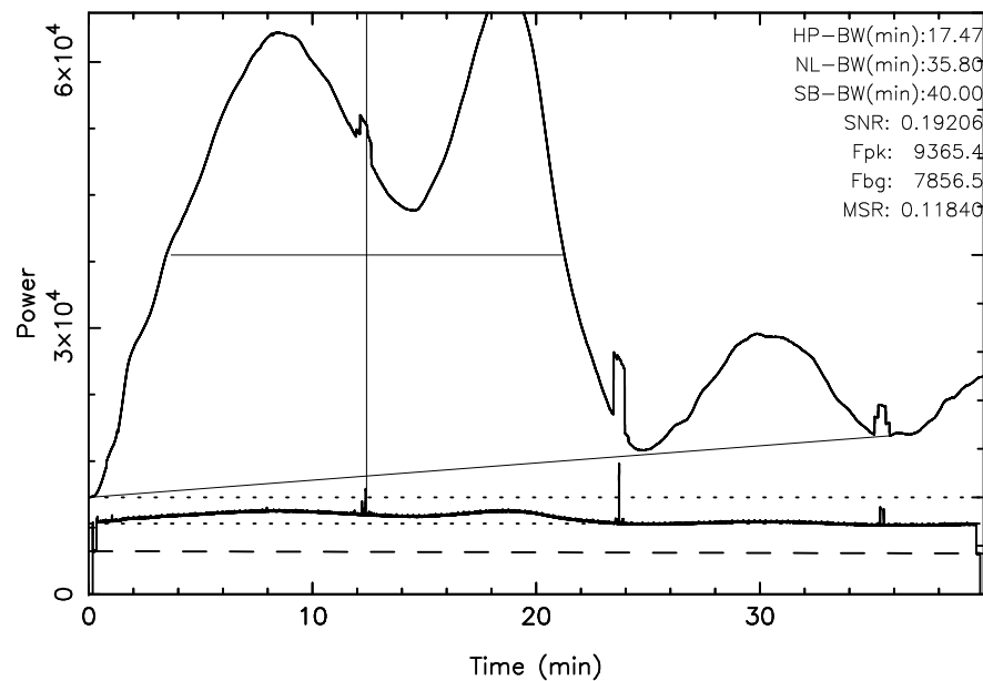
TOYOKAWA 3C123 2024/01/14(014)20:35:18-21:15:18JST
