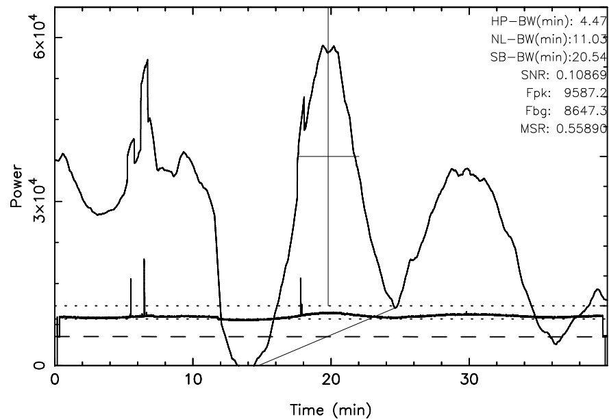
TOYOKAWA 3C123 2024/01/15(015)20:31:22-21:11:22JST
