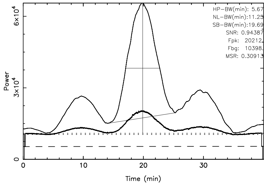
TOYOKAWA 3C144 2024/01/15(015)21:28:35-22:08:35JST
