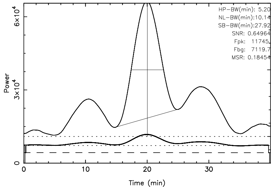
TOYOKAWA 3C274 2024/01/15(015)04:27:27-05:07:27JST
