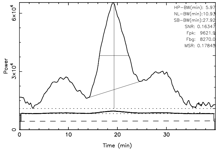
TOYOKAWA 3C157 2024/01/15(015)22:11:59-22:51:59JST
