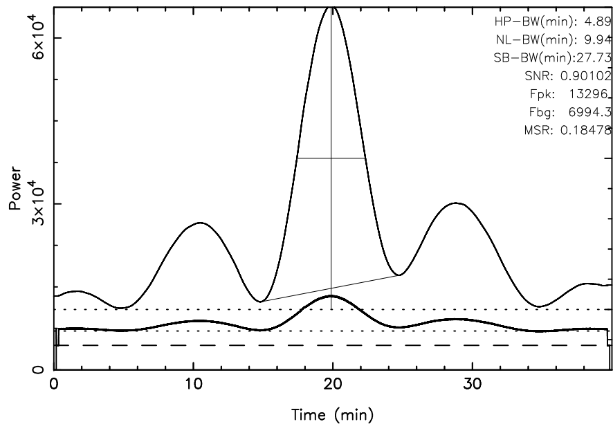
TOYOKAWA 3C274 2024/01/22(022)03:59:55-04:39:55JST
