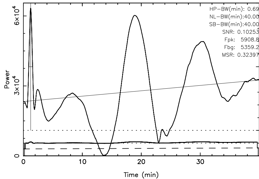
TOYOKAWA 3C157 2024/01/22(022)21:44:28-22:24:28JST
