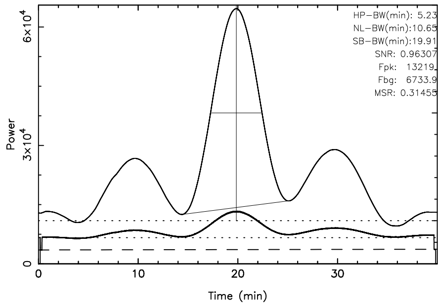
TOYOKAWA 3C144 2024/01/22(022)21:01:03-21:41:03JST
