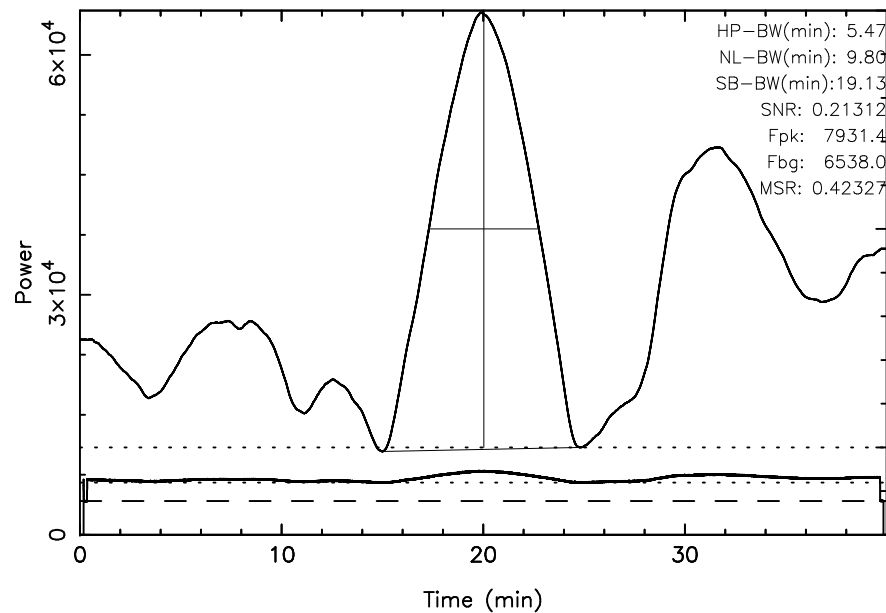
TOYOKAWA 3C123 2024/01/22(022)20:03:51-20:43:51JST
