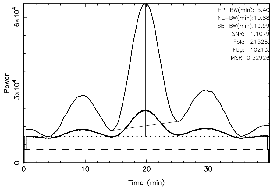
TOYOKAWA 3C144 2024/01/25(025)20:49:16-21:29:16JST
