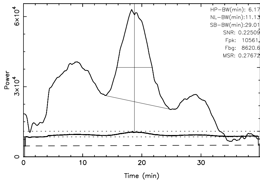
TOYOKAWA 3C157 2024/01/25(025)21:32:40-22:12:40JST
