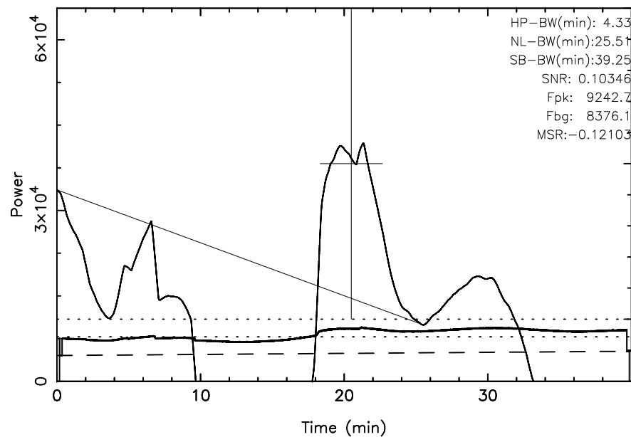
TOYOKAWA 3C123 2024/01/25(025)19:52:03-20:32:03JST
