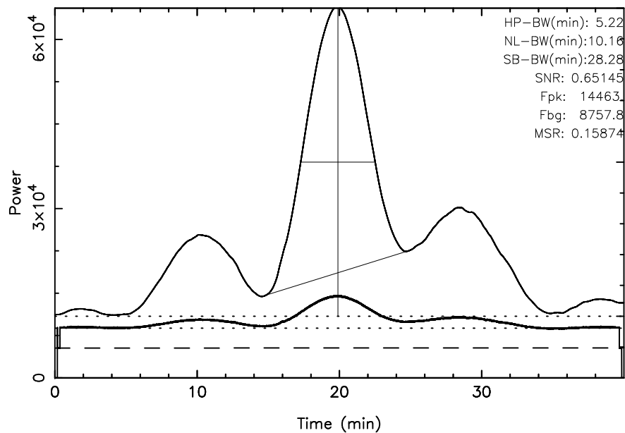
TOYOKAWA 3C274 2024/01/25(025)03:48:08-04:28:08JST
