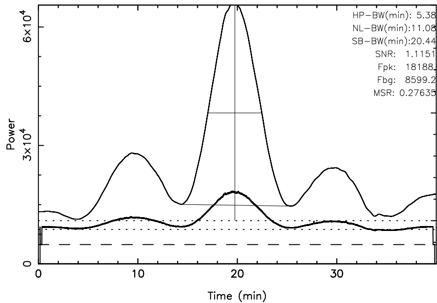
TOYOKAWA 3C144 2024/01/26(026)20:45:20-21:25:20JST
