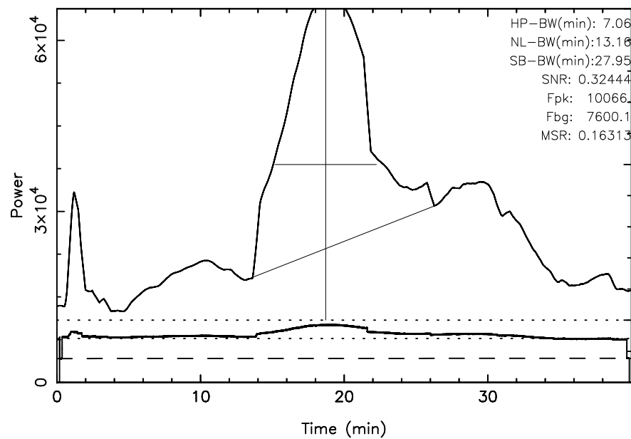
TOYOKAWA 3C157 2024/01/27(027)21:24:48-22:04:48JST
