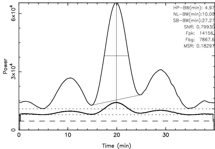
TOYOKAWA 3C274 2024/01/27(027)03:40:16-04:20:16JST
