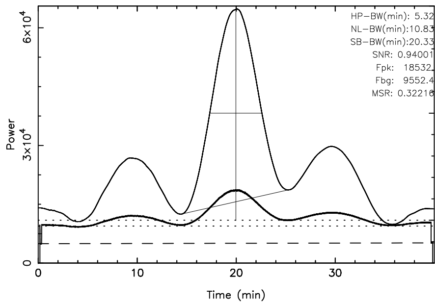
TOYOKAWA 3C144 2024/01/27(027)20:41:24-21:21:24JST
