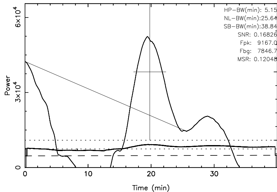
TOYOKAWA 3C123 2024/01/27(027)19:44:11-20:24:11JST
