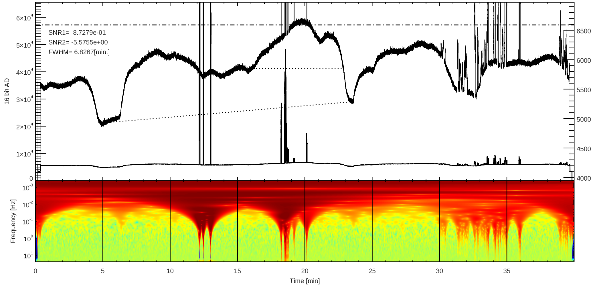
C 3C123 (/home4/archive/swift/dat/2024/02/T20240213183723.dat)
