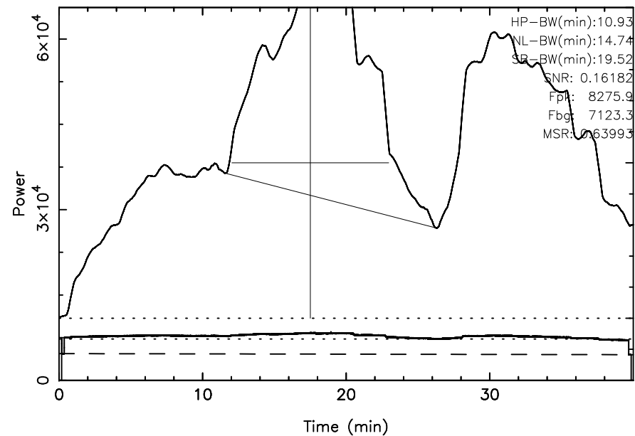
TOYOKAWA 3C295 2024/01/31(031)05:04:25-05:44:25JST
