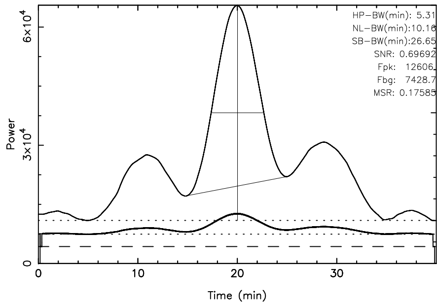
TOYOKAWA 3C274 2024/01/31(031)03:24:32-04:04:32JST
