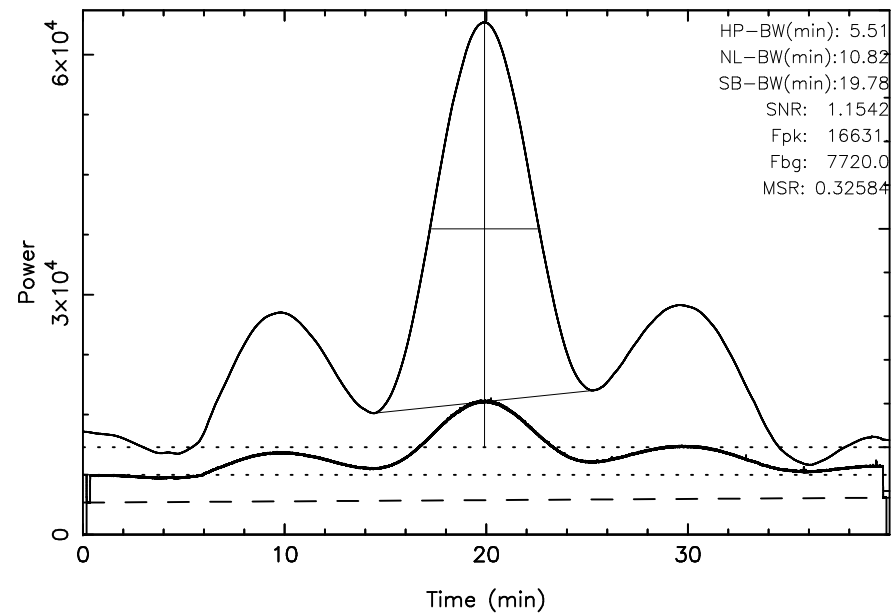
TOYOKAWA 3C144 2024/01/31(031)20:25:40-21:05:40JST
