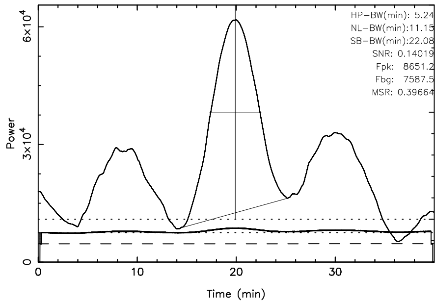
TOYOKAWA 3C123 2024/01/31(031)19:28:27-20:08:27JST
