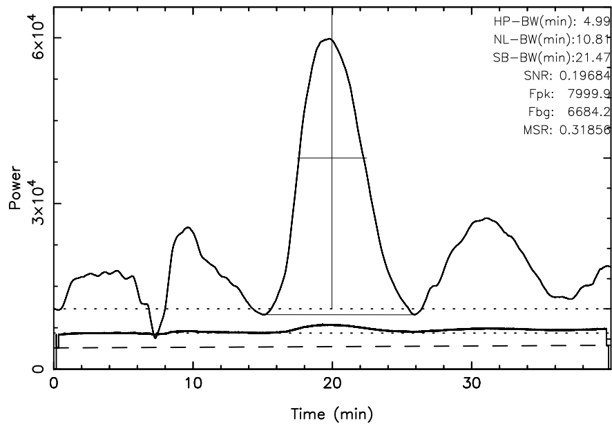
TOYOKAWA 3C123 2024/02/01(032)19:24:32-20:04:32JST
