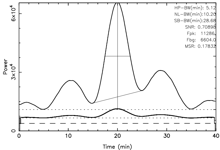
TOYOKAWA 3C274 2024/02/14(045)02:29:30-03:09:30JST
