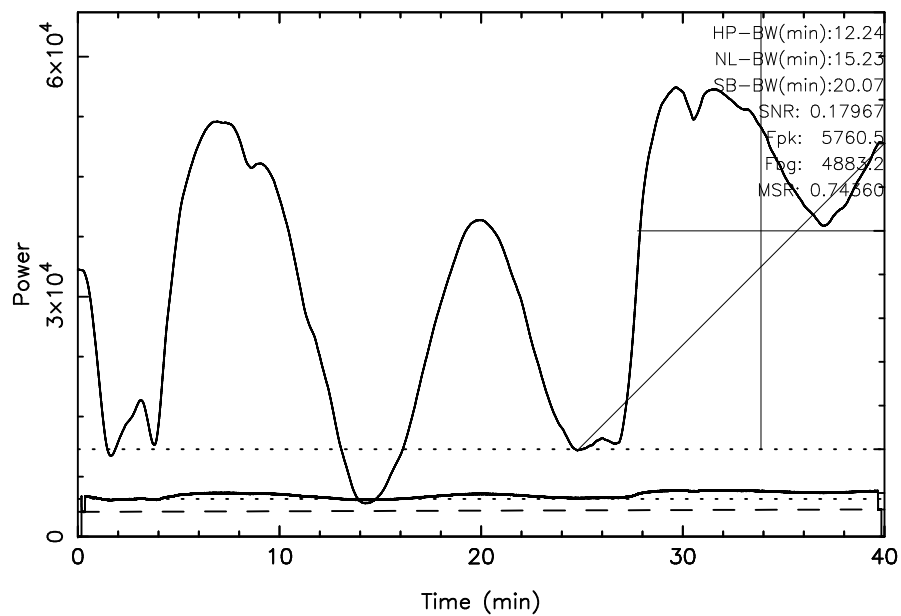
TOYOKAWA 3C123 2024/02/14(045)18:33:25-19:13:25JST
