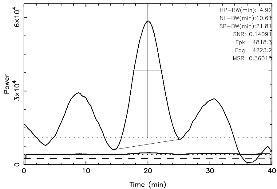
TOYOKAWA 3C123 2024/02/20(051)18:09:49-18:49:49JST
