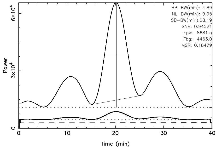
TOYOKAWA 3C274 2024/02/20(051)02:05:54-02:45:54JST
