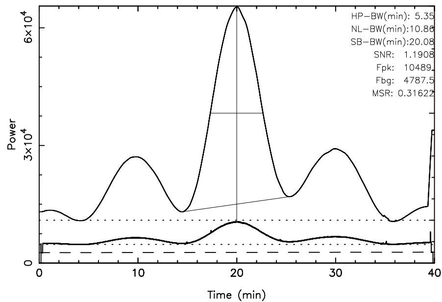
TOYOKAWA 3C144 2024/02/20(051)19:07:02-19:47:02JST
