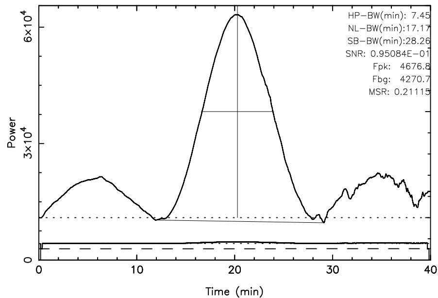
TOYOKAWA 3C295 2024/02/20(051)03:45:47-04:25:47JST
