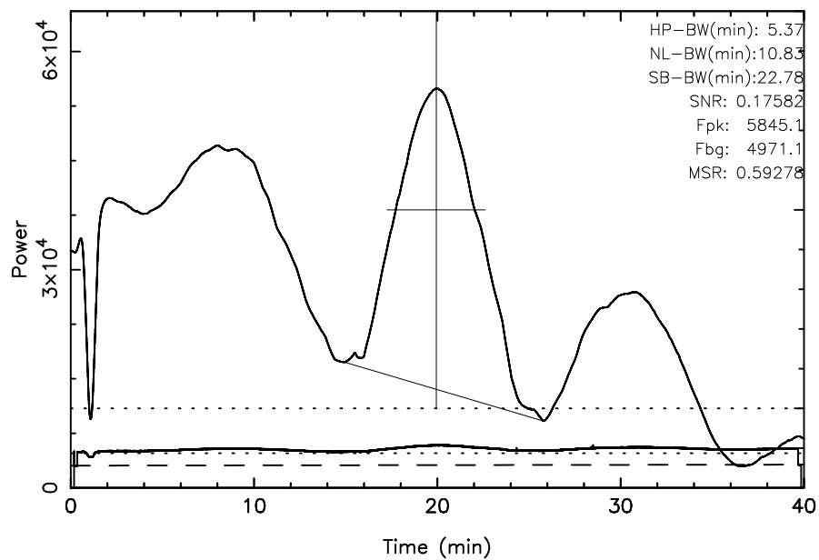
TOYOKAWA 3C123 2024/02/22(053)18:01:58-18:41:58JST
