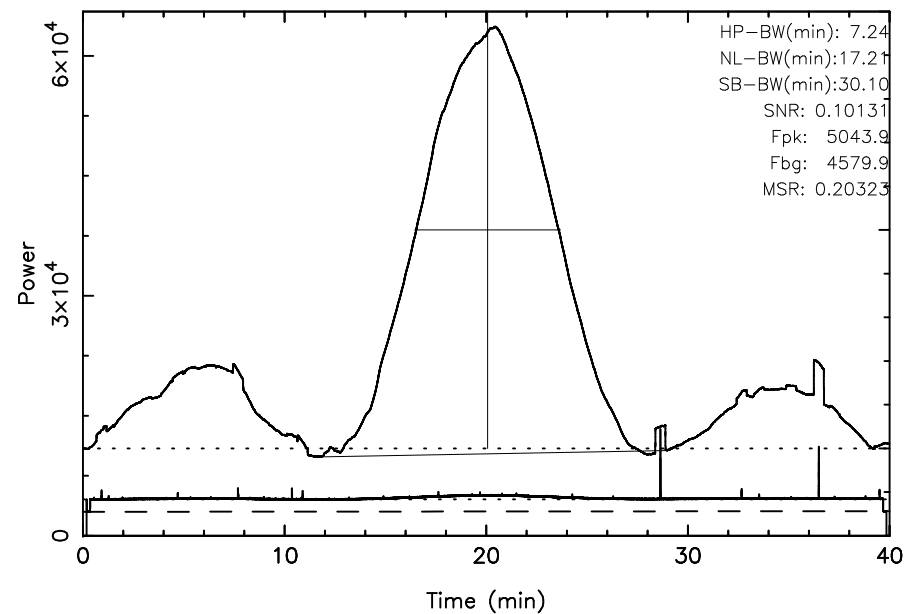
TOYOKAWA 3C295 2024/02/22(053)03:37:55-04:17:55JST
