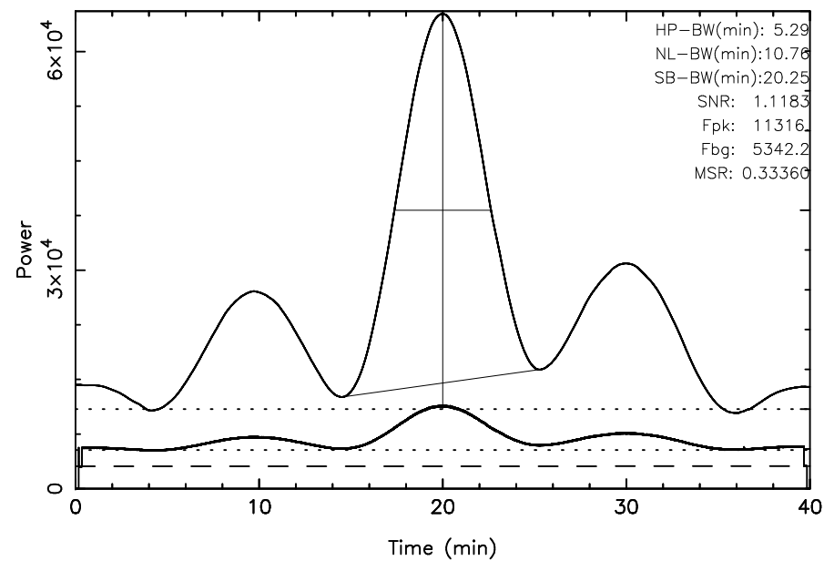
TOYOKAWA 3C144 2024/02/22(053)18:59:10-19:39:10JST
