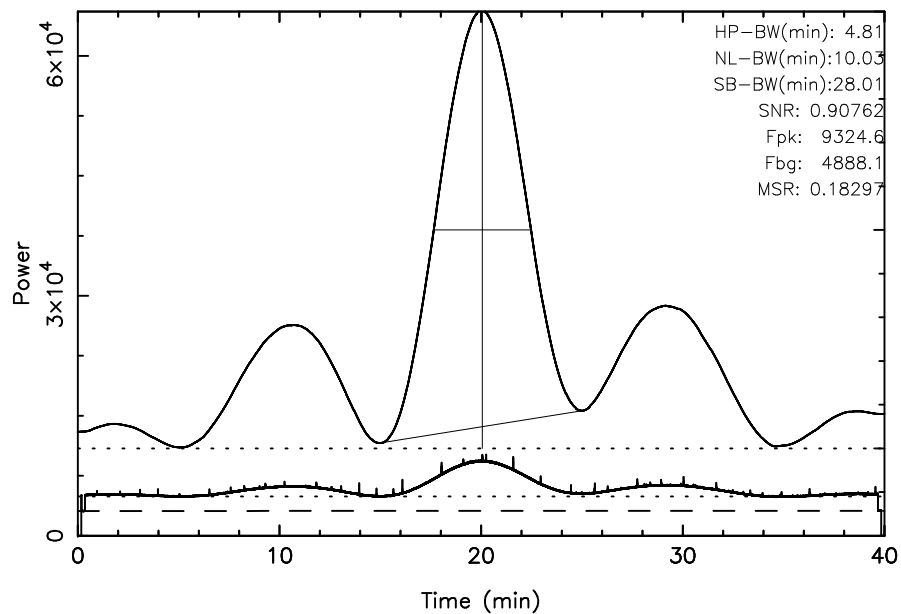
TOYOKAWA 3C274 2024/02/22(053)01:58:02-02:38:02JST
