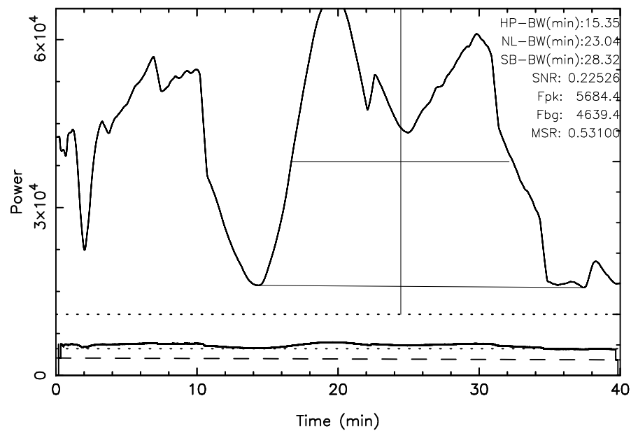
TOYOKAWA 3C157 2024/02/23(054)19:38:39-20:18:39JST
