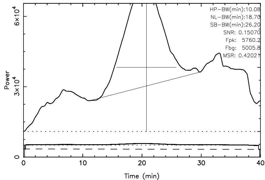
TOYOKAWA 3C295 2024/02/23(054)03:33:59-04:13:59JST
