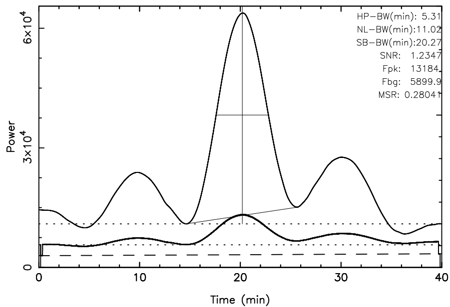
TOYOKAWA 3C144 2024/02/23(054)18:55:14-19:35:14JST
