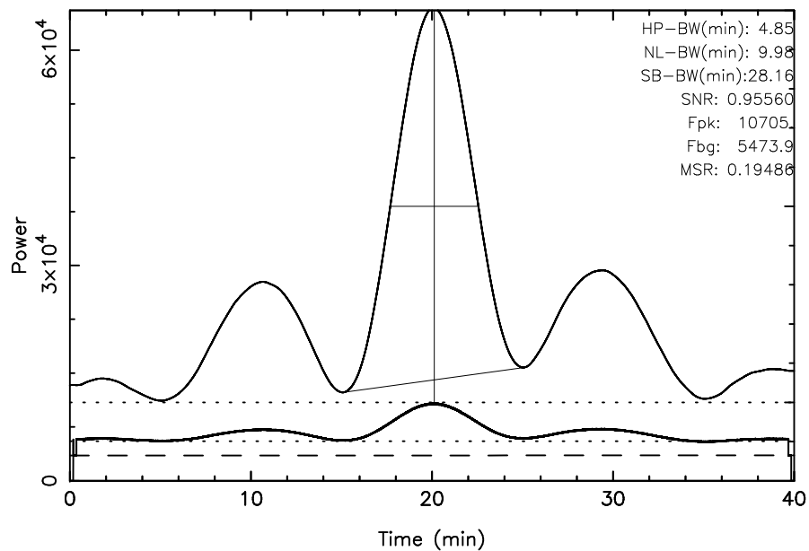
TOYOKAWA 3C274 2024/02/23(054)01:54:07-02:34:07JST
