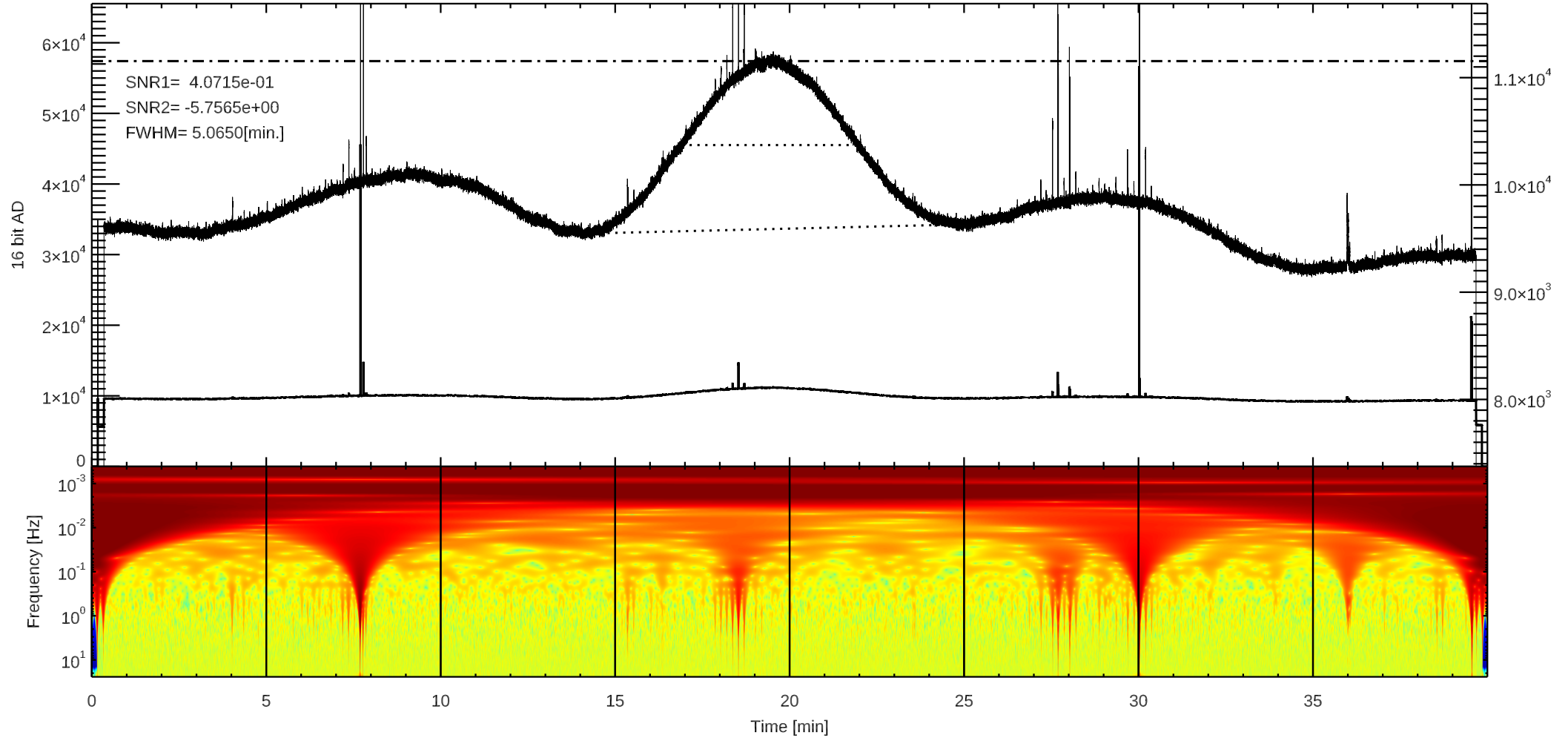
C 3C157 (/home4/archive/swift/dat/2024/03/T20240323174441.dat)
