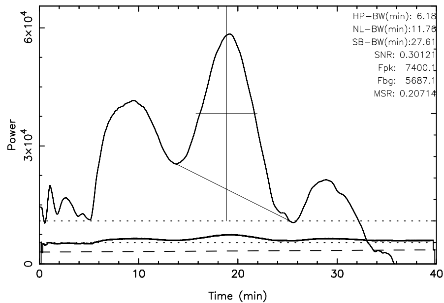
TOYOKAWA 3C157 2024/03/01(061)19:11:08-19:51:08JST
