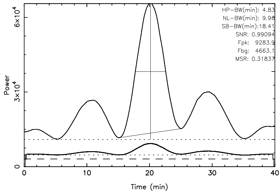
TOYOKAWA 3C274 2024/03/01(061)01:26:35-02:06:35JST
