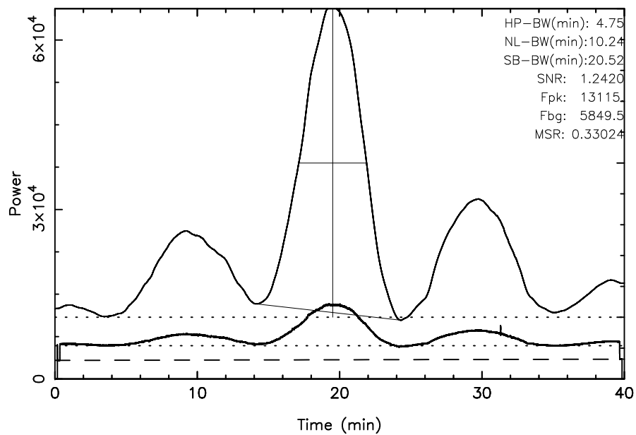
TOYOKAWA 3C144 2024/03/01(061)18:27:43-19:07:43JST
