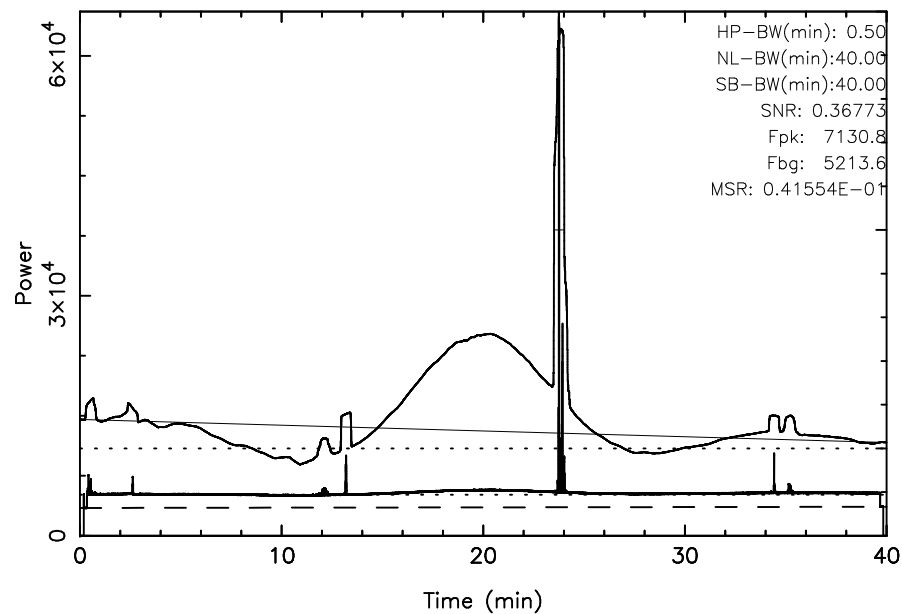
TOYOKAWA 3C295 2024/03/01(061)03:06:28-03:46:28JST
