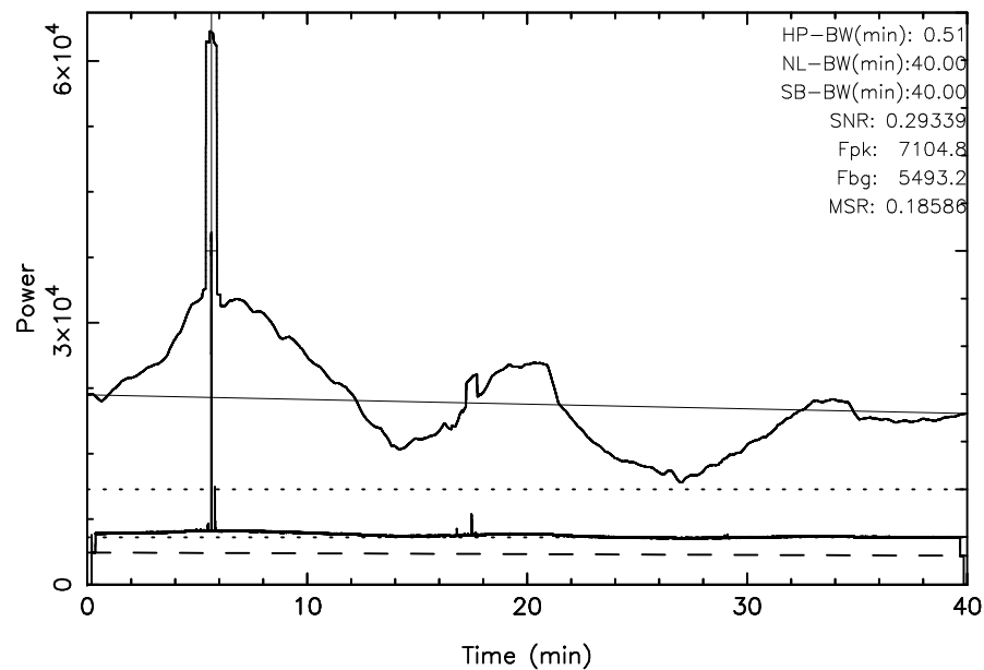
TOYOKAWA 3C295 2024/03/02(062)03:02:32-03:42:32JST
