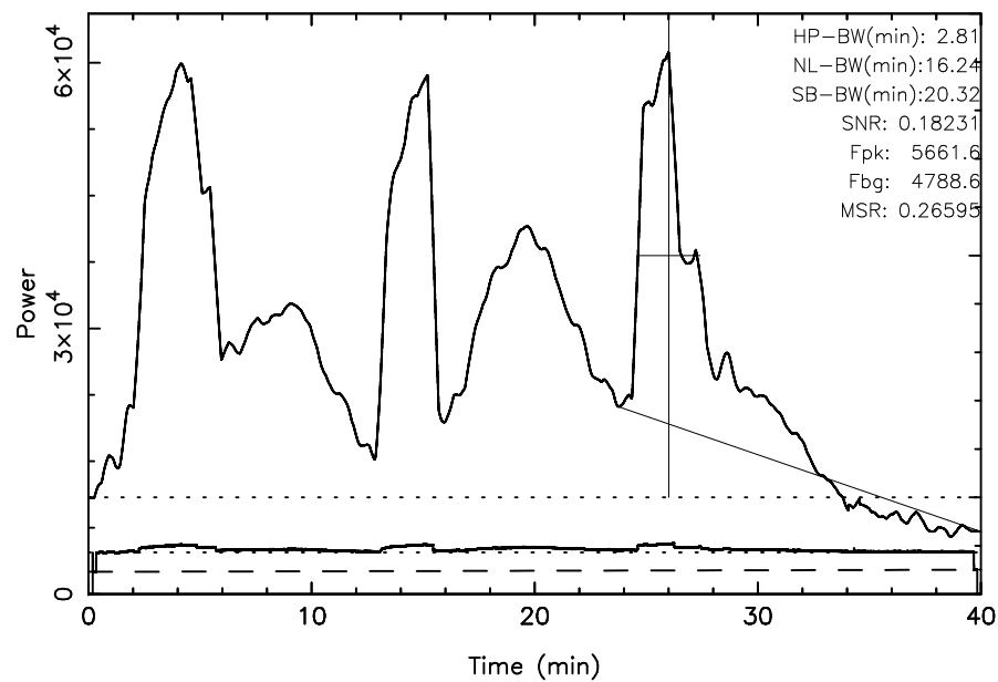
TOYOKAWA 3C157 2024/03/02(062)19:07:12-19:47:12JST
