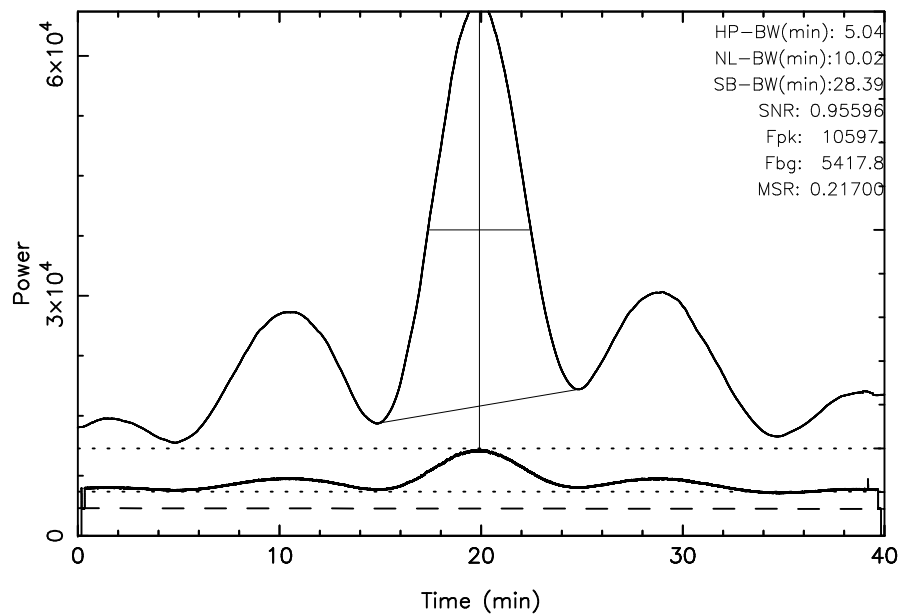
TOYOKAWA 3C274 2024/03/02(062)01:22:39-02:02:39JST
