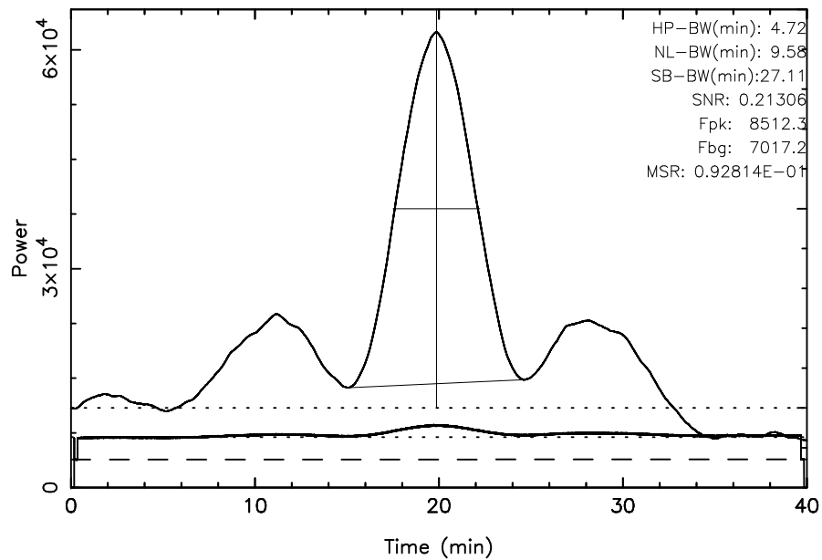
TOYOKAWA 3C348 2024/03/05(065)05:30:27-06:10:27JST
