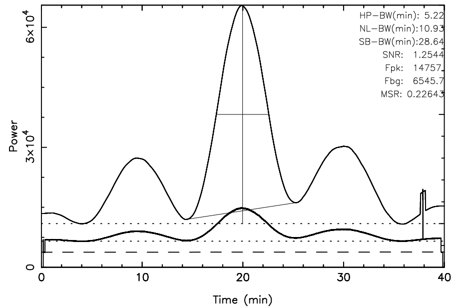
TOYOKAWA 3C144 2024/03/05(065)18:12:00-18:52:00JST
