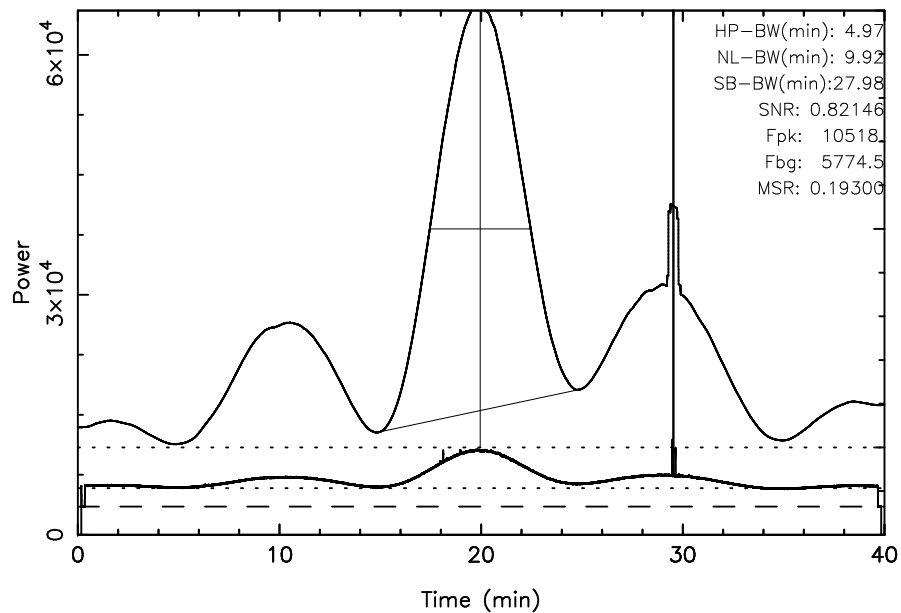
TOYOKAWA 3C274 2024/03/05(065)01:10:52-01:50:52JST
