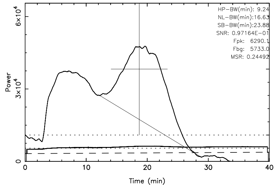
TOYOKAWA 3C295 2024/03/05(065)02:50:44-03:30:44JST
