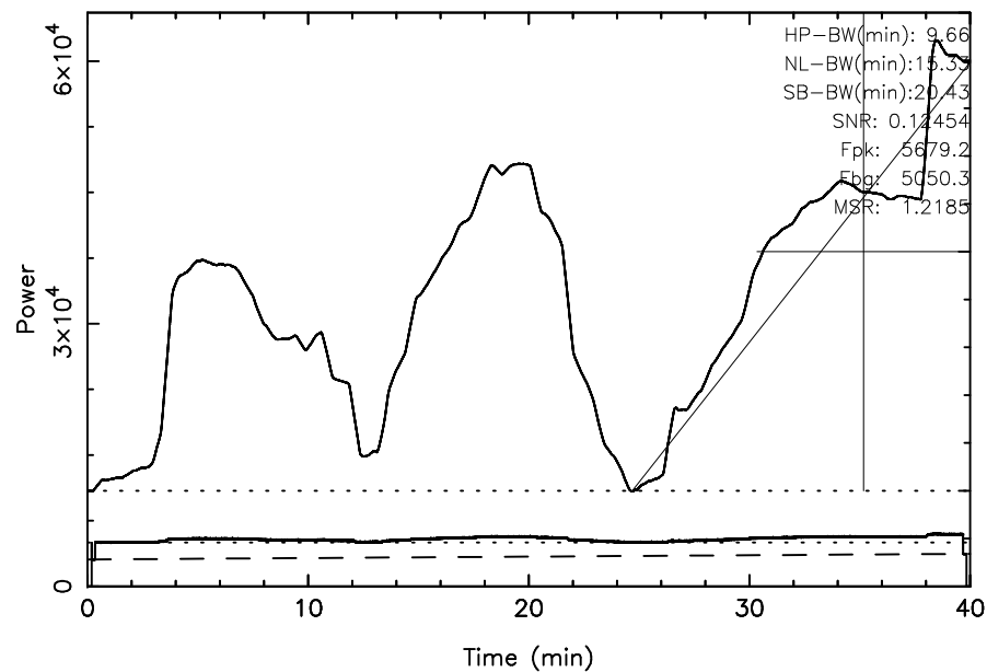
TOYOKAWA 3C295 2024/03/09(069)02:35:00-03:15:00JST
