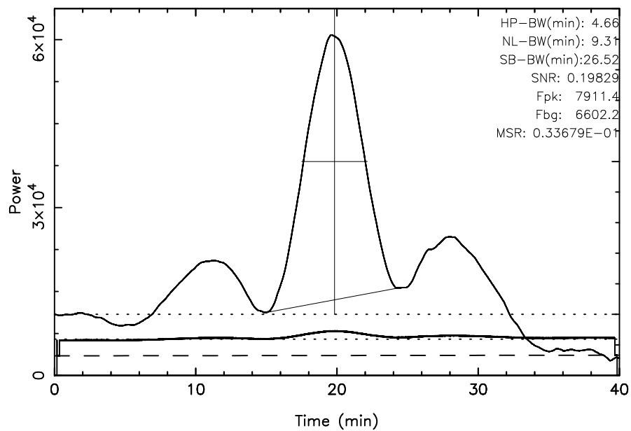
TOYOKAWA 3C348 2024/03/09(069)05:14:43-05:54:43JST
