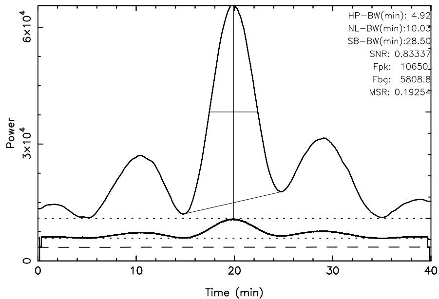
TOYOKAWA 3C274 2024/03/09(069)00:55:08-01:35:08JST
