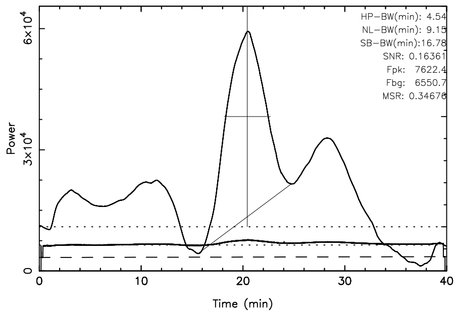
TOYOKAWA 3C348 2024/03/11(071)05:06:51-05:46:51JST
