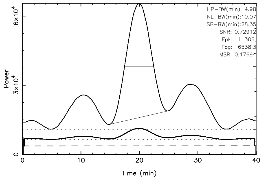
TOYOKAWA 3C274 2024/03/11(071)00:47:16-01:27:16JST
