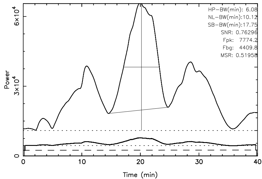
TOYOKAWA 3C144 2024/03/11(071)17:48:24-18:28:24JST
