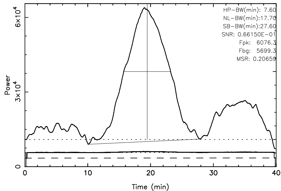
TOYOKAWA 3C295 2024/03/11(071)02:27:08-03:07:08JST
