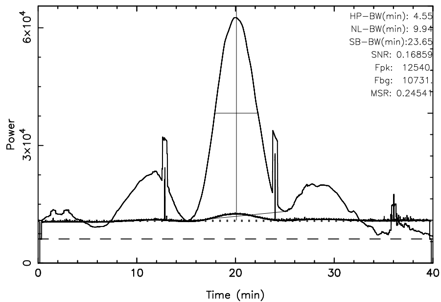
TOYOKAWA 3C348 2024/03/13(073)04:58:59-05:38:59JST
