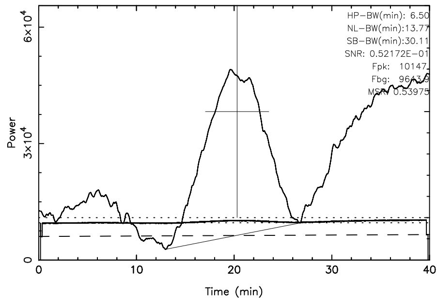
TOYOKAWA 3C295 2024/03/13(073)02:19:17-02:59:17JST
