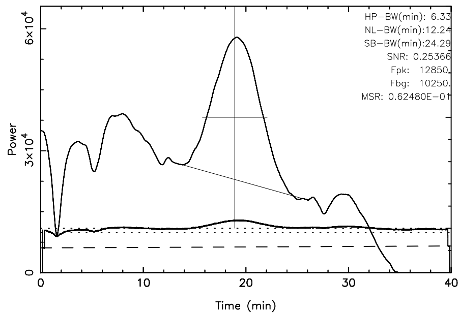
TOYOKAWA 3C157 2024/03/13(073)18:23:57-19:03:57JST
