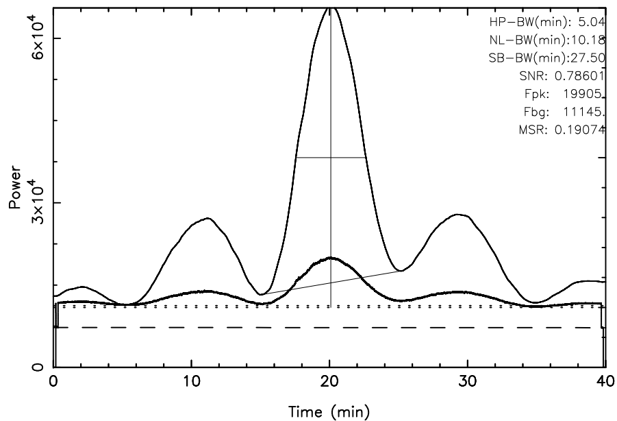
TOYOKAWA 3C274 2024/03/13(073)00:39:24-01:19:24JST
