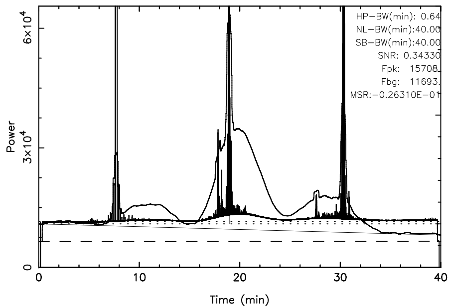
TOYOKAWA 3C348 2024/03/21(081)04:27:32-05:07:32JST
