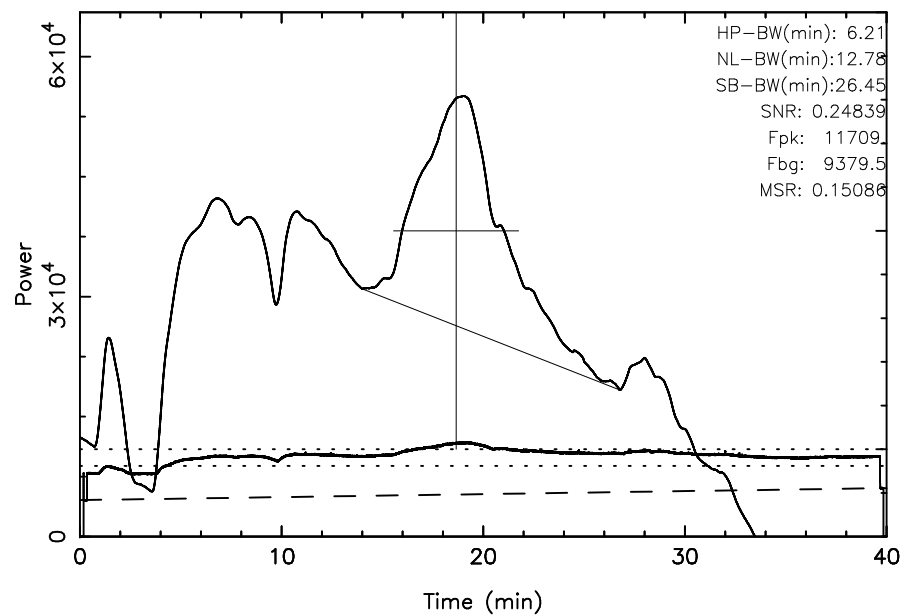
TOYOKAWA 3C157 2024/03/21(081)17:52:30-18:32:30JST
