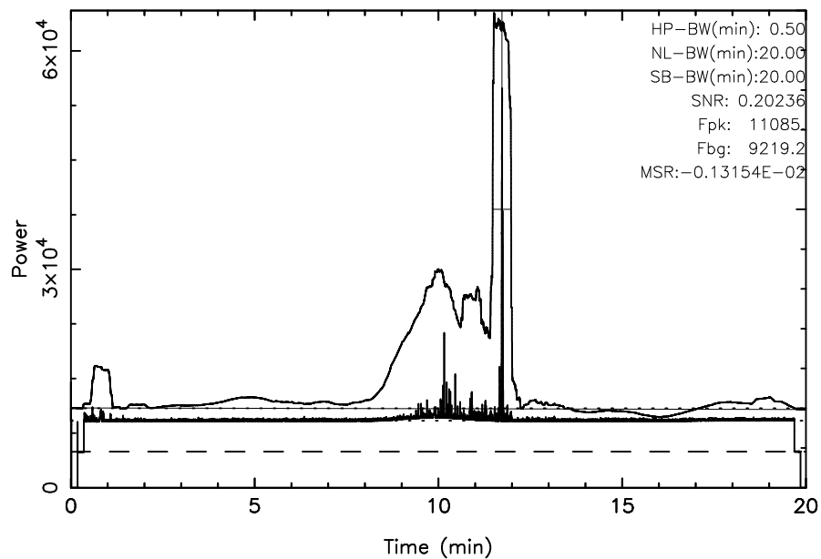
FUJI 3C348 2024/04/15(106)02:59:15-03:19:15JST
