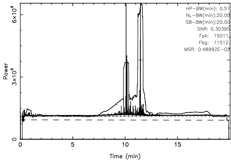
KISO 3C348 2024/04/15(106)02:59:15-03:19:15JST
