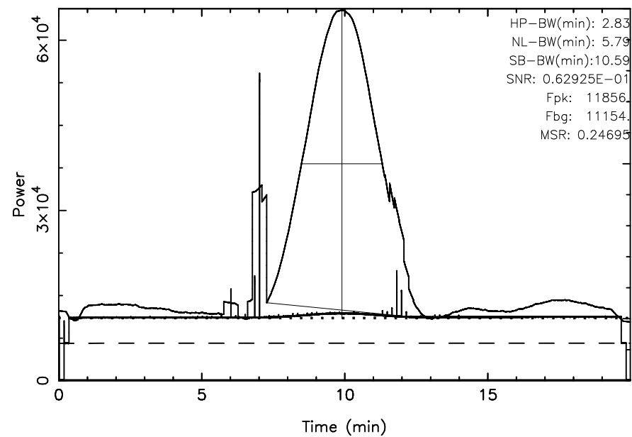
KISO 3C348 2024/04/21(112)02:35:39-02:55:38JST
