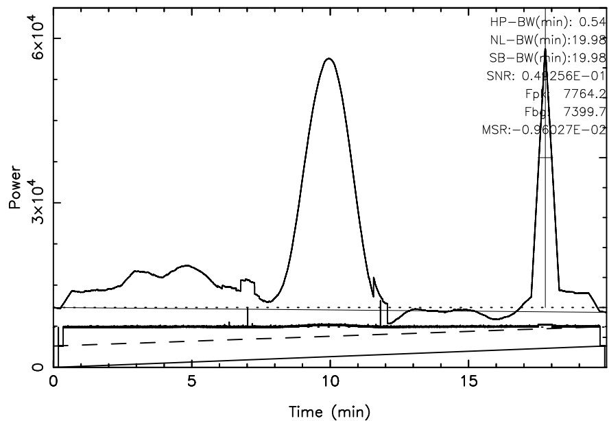
FUJI 3C348 2024/04/21(112)02:35:39-02:55:38JST
