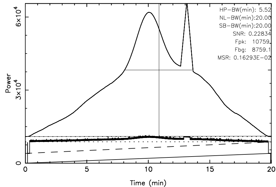
FUJI 3C392 2024/04/21(112)04:40:17-05:00:17JST
