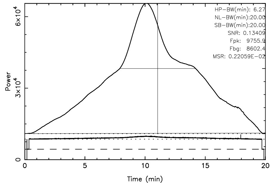
FUJI 3C392 2024/04/25(116)04:24:33-04:44:33JST
