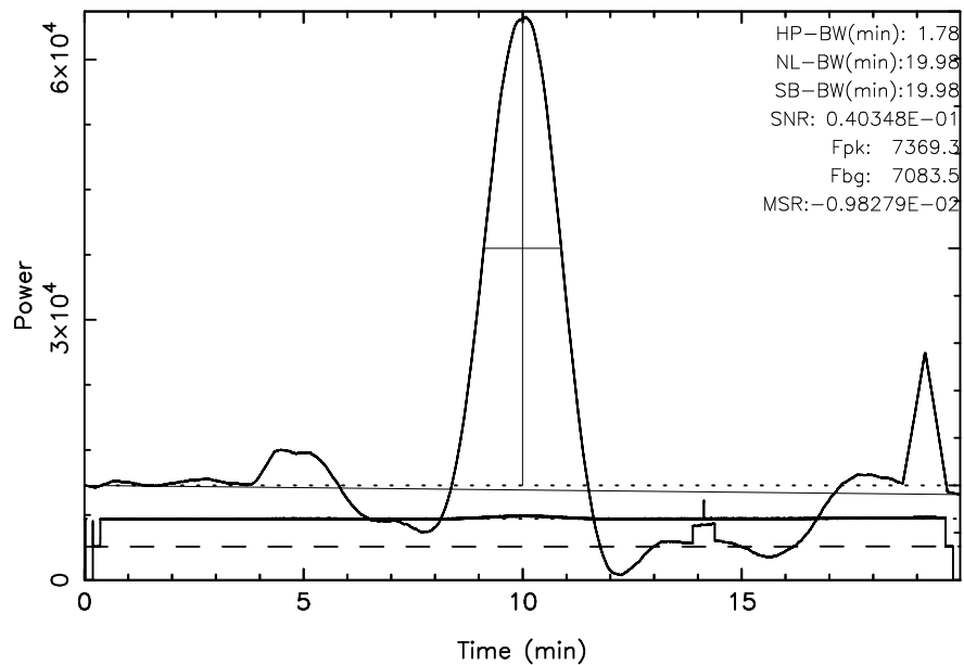
FUJI 3C348 2024/04/29(120)02:04:12-02:24:11JST
