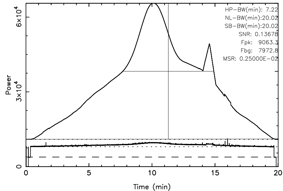
FUJI 3C392 2024/04/29(120)04:08:50-04:28:51JST
