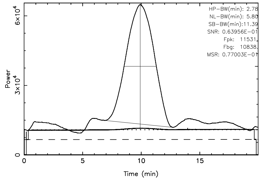
KISO 3C348 2024/04/29(120)02:04:12-02:24:11JST
