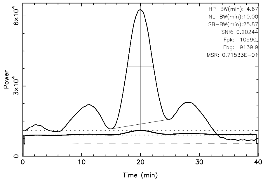
TOYOKAWA 3C348 2024/04/29(120)01:54:12-02:34:12JST
