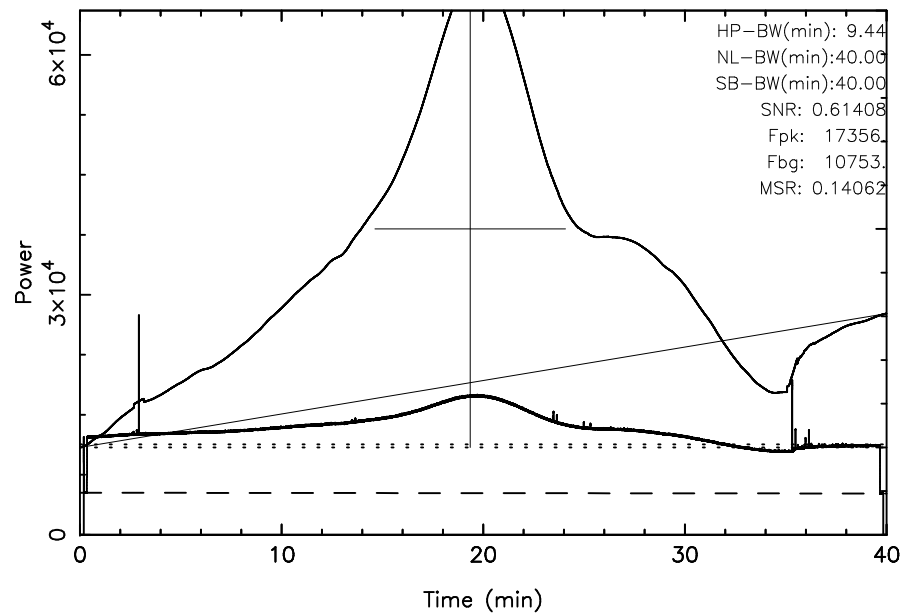
TOYOKAWA 3C392 2024/04/29(120)03:58:51-04:38:51JST
