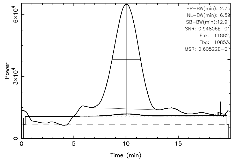
KISO 3C348 2024/04/30(121)02:00:16-02:20:15JST
