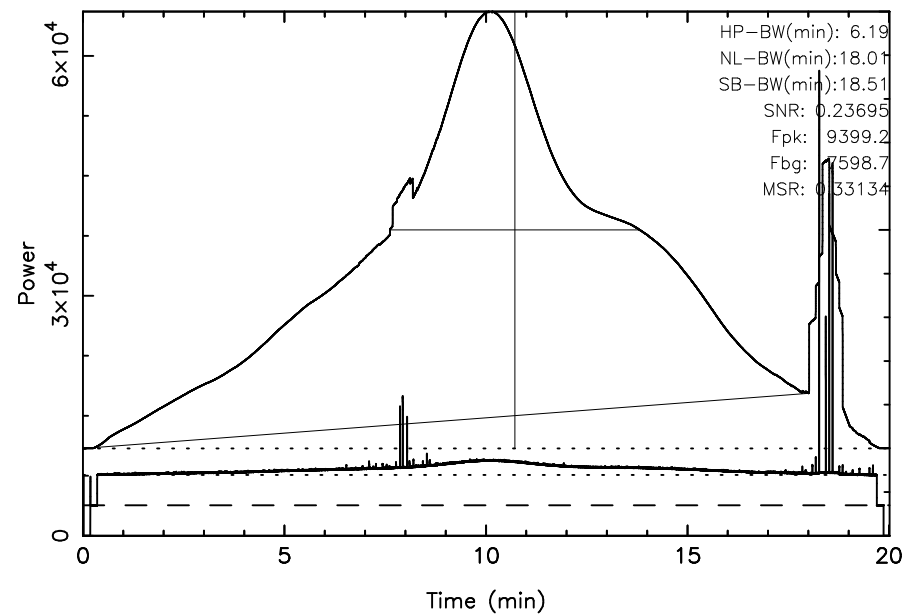
FUJI 3C392 2024/04/30(121)04:04:54-04:24:55JST
