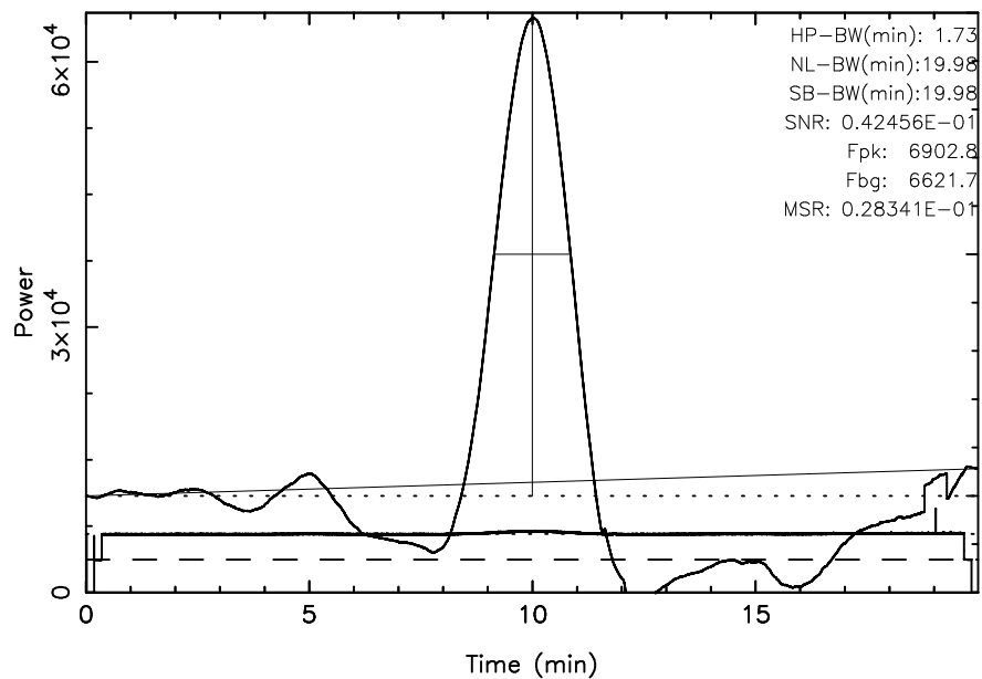
FUJI 3C348 2024/04/30(121)02:00:16-02:20:15JST
