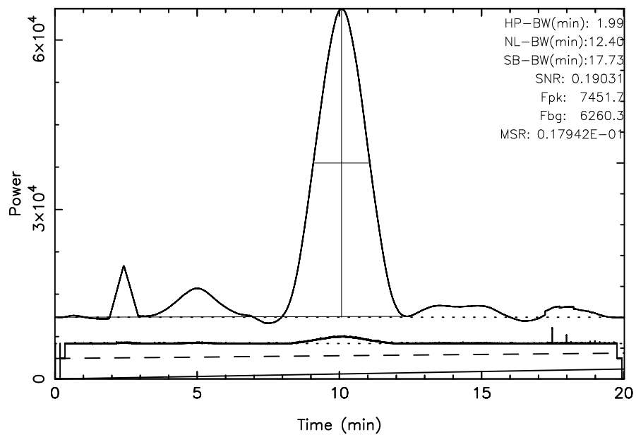
FUJI 3C274 2024/05/04(125)21:21:01-21:41:02JST
