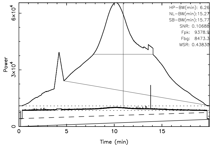
FUJI 3C392 2024/05/04(125)03:49:11-04:09:10JST
