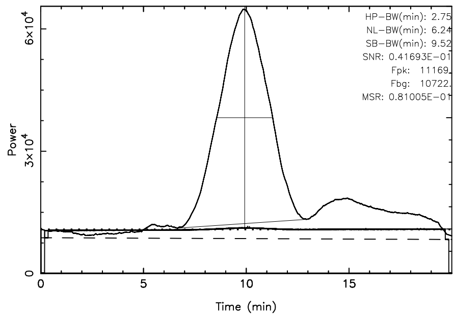
KISO 3C348 2024/05/04(125)01:44:31-02:04:31JST
