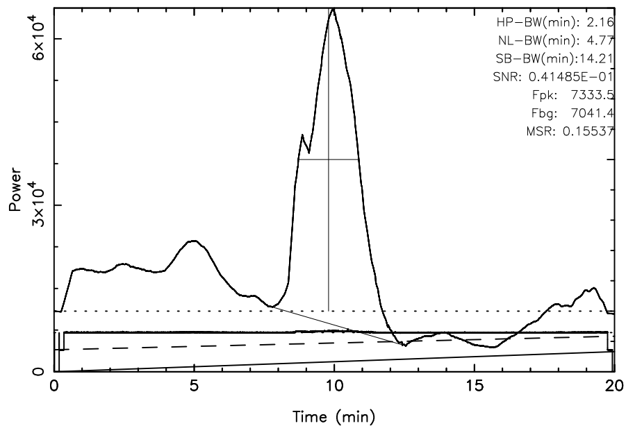
FUJI 3C348 2024/05/04(125)01:44:31-02:04:31JST
