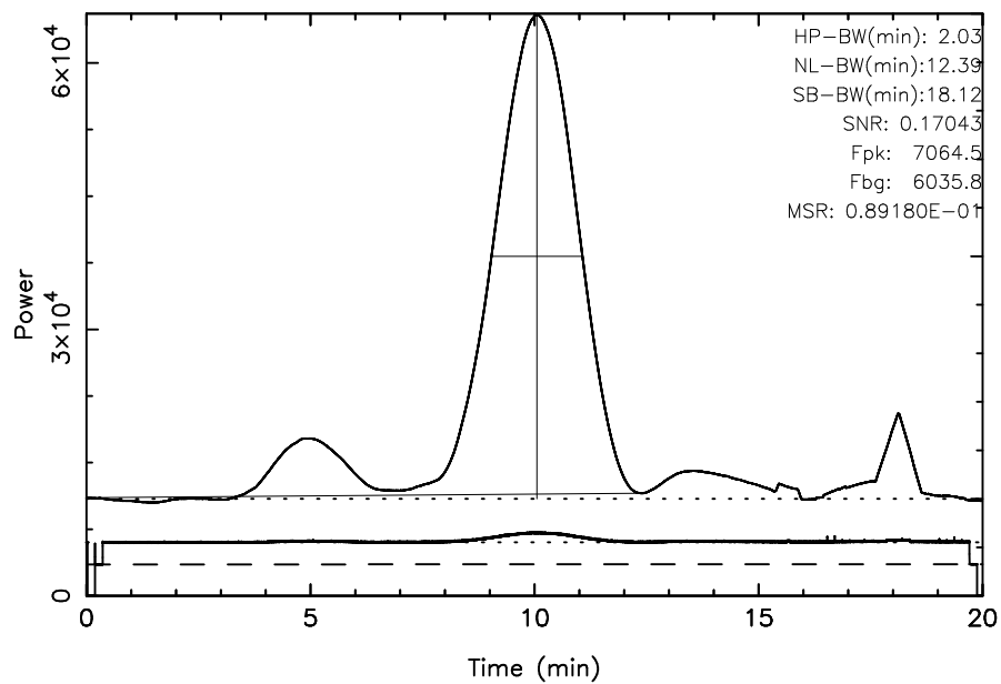
FUJI 3C274 2024/05/08(129)21:05:18-21:25:18JST
