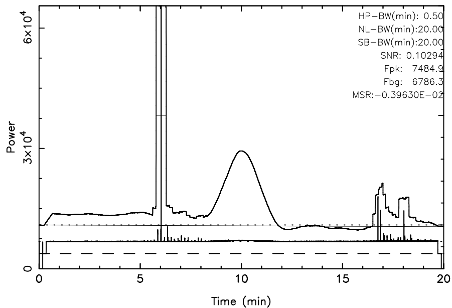
FUJI 3C348 2024/05/08(129)01:28:48-01:48:48JST
