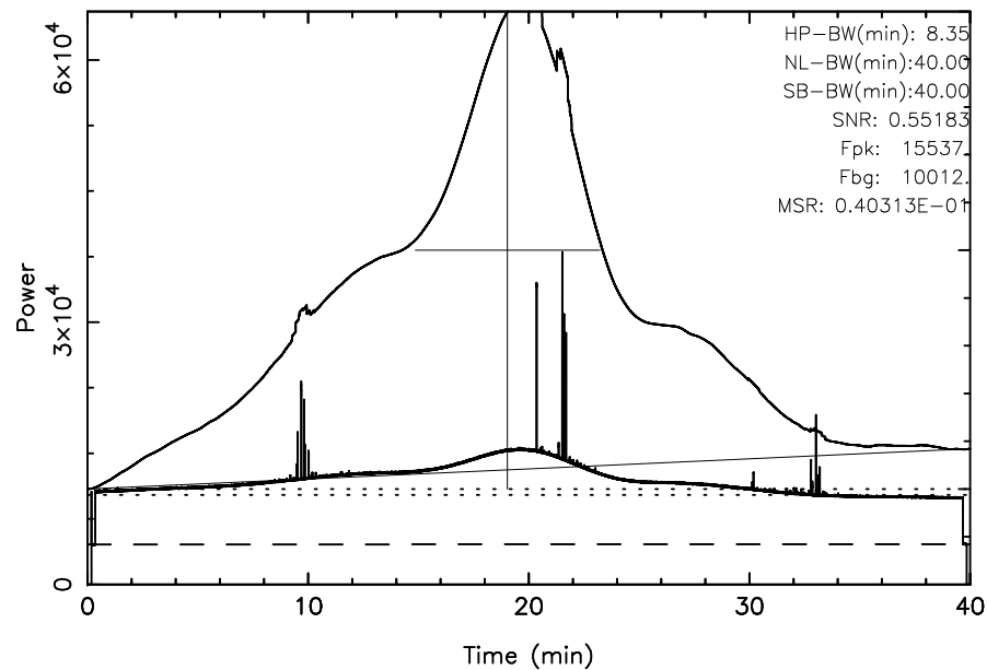
TOYOKAWA 3C392 2024/05/01(122)03:50:59-04:30:59JST
