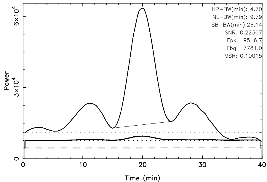
TOYOKAWA 3C348 2024/05/01(122)01:46:20-02:26:20JST
