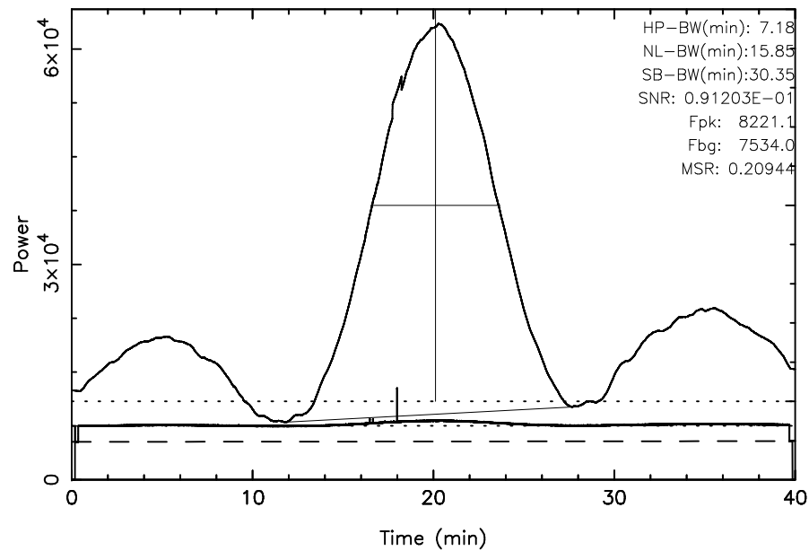
TOYOKAWA 3C295 2024/05/01(122)23:02:41-23:42:41JST
