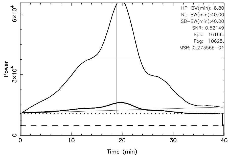
TOYOKAWA 3C392 2024/05/08(129)03:23:28-04:03:28JST
