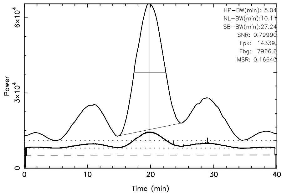
TOYOKAWA 3C274 2024/05/08(129)20:55:18-21:35:18JST
