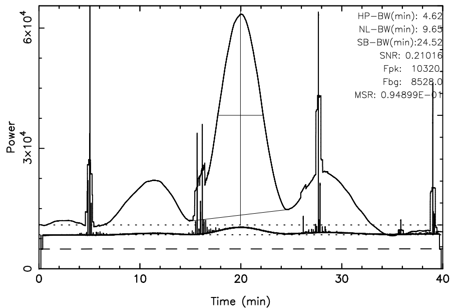
TOYOKAWA 3C348 2024/05/08(129)01:18:49-01:58:49JST
