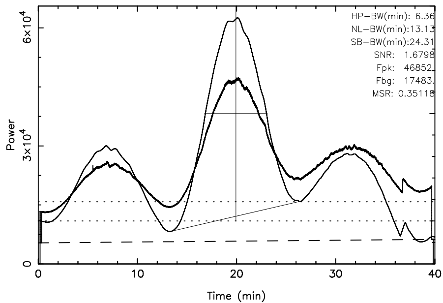
TOYOKAWA 3C405 2024/05/11(132)04:14:29-04:54:29JST
