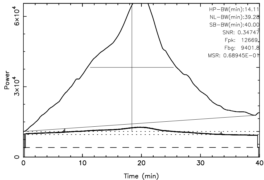
TOYOKAWA 3C392 2024/05/11(132)03:11:40-03:51:40JST
