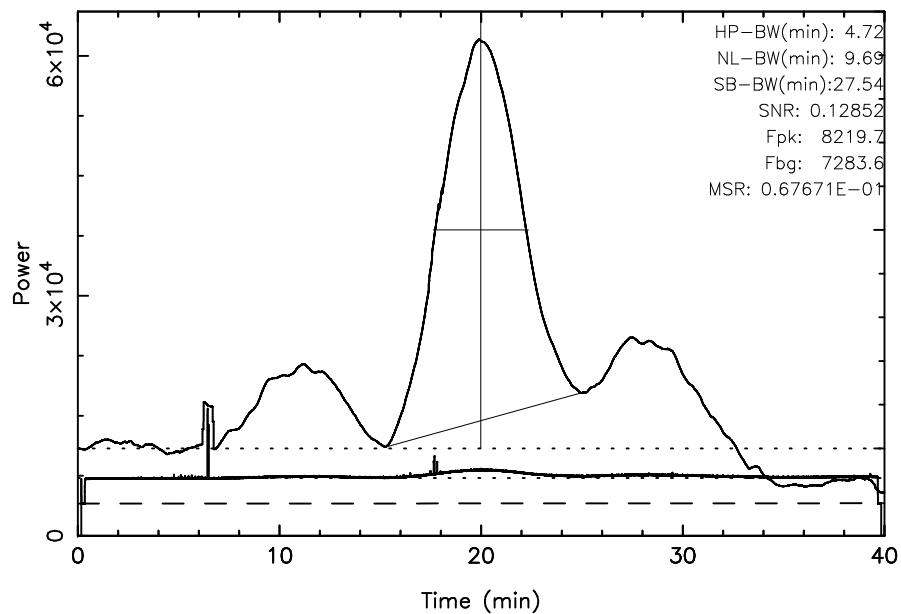
TOYOKAWA 3C348 2024/05/11(132)01:07:01-01:47:01JST
