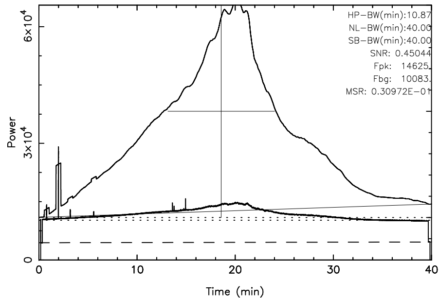
TOYOKAWA 3C392 2024/05/12(133)03:07:44-03:47:44JST
