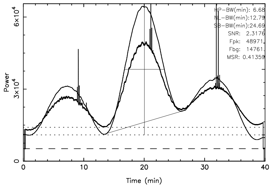
TOYOKAWA 3C405 2024/05/27(148)03:11:34-03:51:34JST
