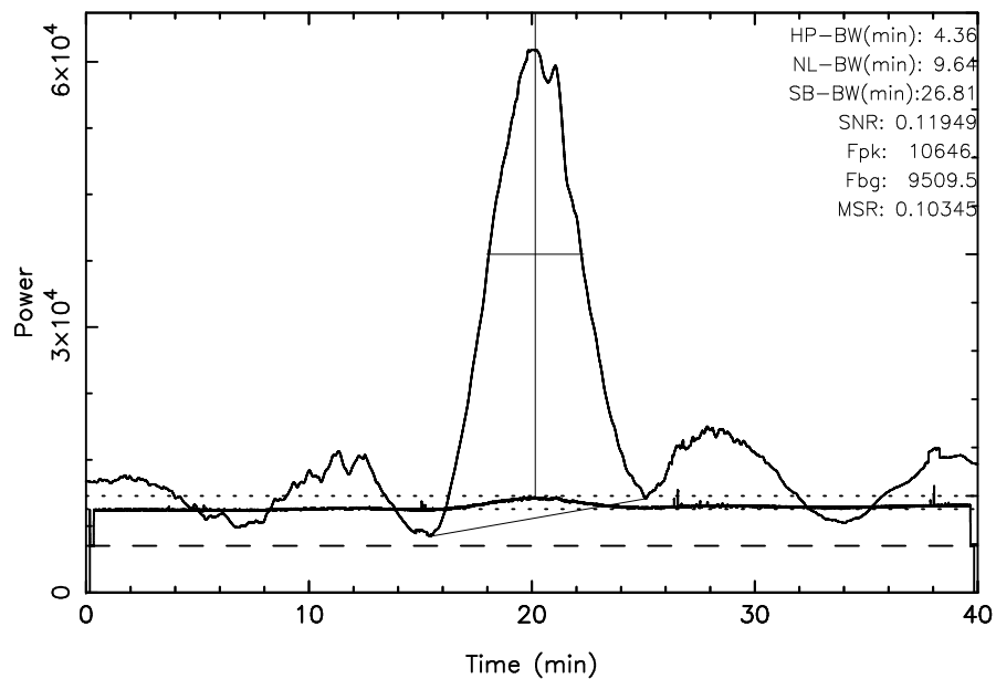
TOYOKAWA 3C353 2024/05/27(148)00:33:27-01:13:27JST
