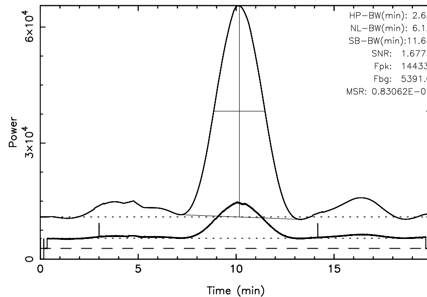
FUJI 3C405 2024/06/12(164)02:18:40-02:38:39JST
