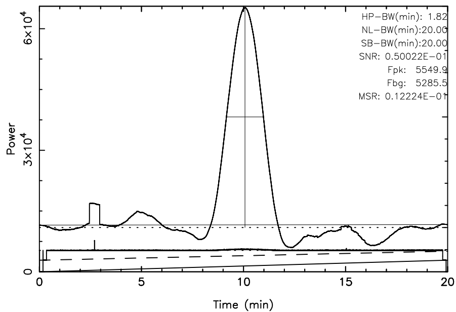
FUJI 3C348 2024/06/15(167)22:55:28-23:15:28JST
