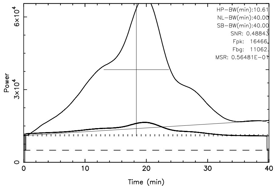
TOYOKAWA 3C392 2024/06/09(161)01:17:39-01:57:39JST
