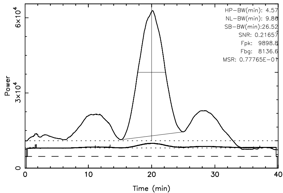
TOYOKAWA 3C348 2024/06/09(161)23:09:04-23:49:04JST
