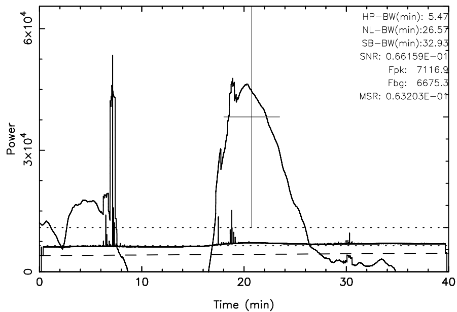
TOYOKAWA 3C295 2024/06/09(161)20:29:21-21:09:21JST
