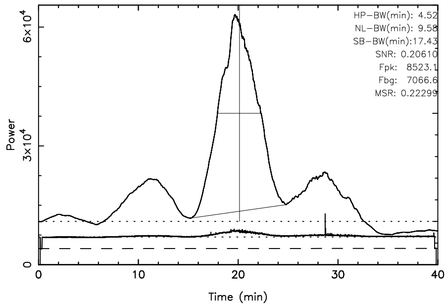
TOYOKAWA 3C348 2024/06/26(178)22:02:14-22:42:14JST
