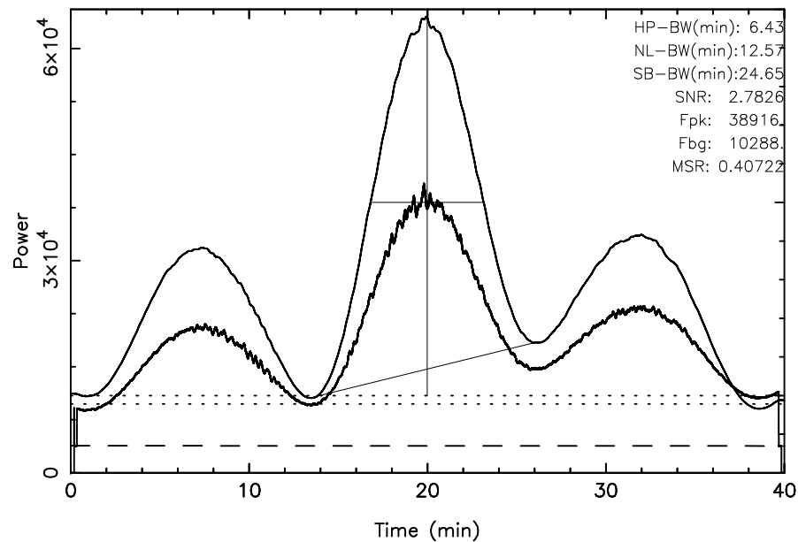
TOYOKAWA 3C405 2024/06/26(178)01:13:37-01:53:37JST
