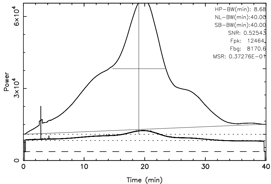
TOYOKAWA 3C392 2024/06/26(178)00:10:48-00:50:48JST
