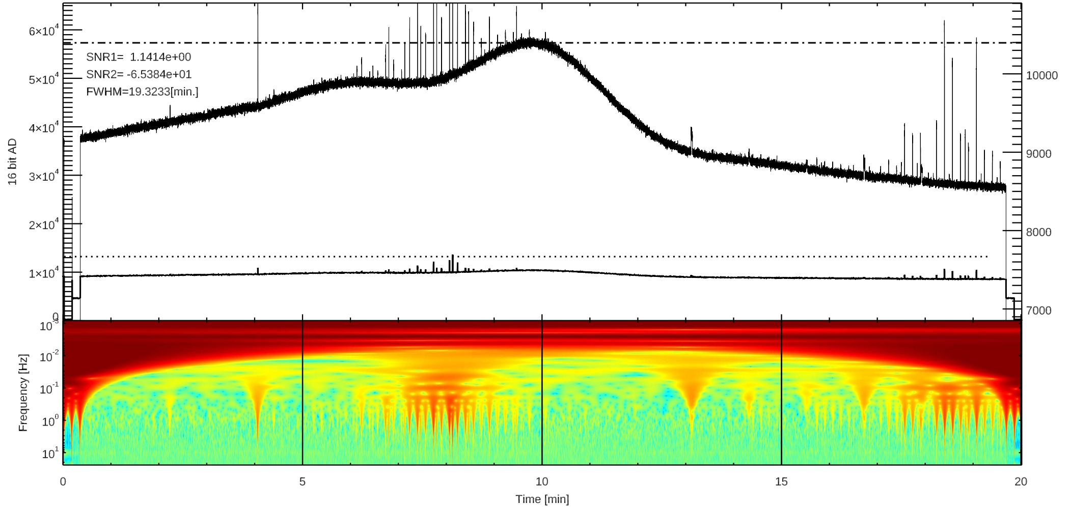
C 3C392 (/home4/archive/kit/dat/2024/07/K20240719224625.dat)
