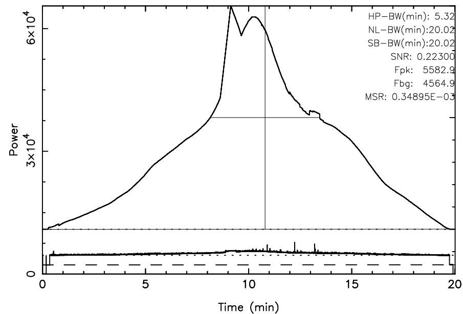
FUJI 3C392 2024/08/08(221)21:27:48-21:47:49JST
