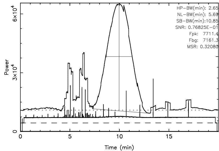
KISO 3C348 2024/08/22(235)18:28:07-18:48:07JST
