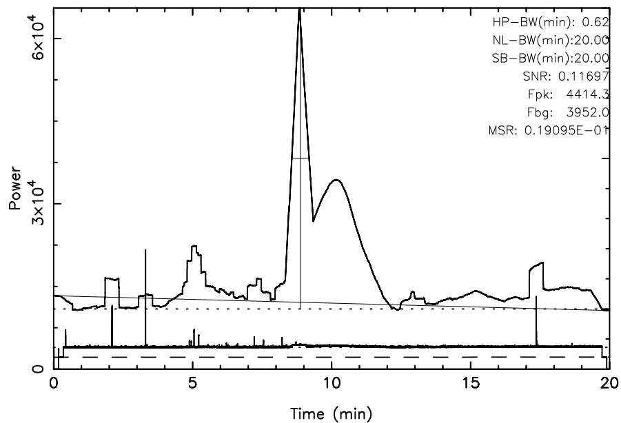
FUJI 3C348 2024/08/22(235)18:28:07-18:48:07JST
