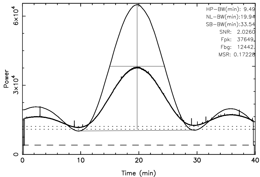
TOYOKAWA 3C461 2024/08/07(220)01:52:05-02:32:05JST
