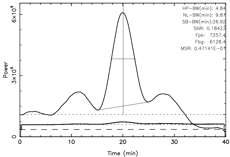
TOYOKAWA 3C348 2024/08/07(220)19:17:06-19:57:06JST
