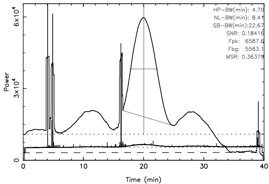
TOYOKAWA 3C348 2024/08/22(235)18:18:07-18:58:07JST
