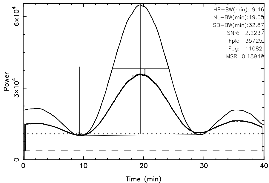
TOYOKAWA 3C461 2024/08/22(235)00:53:07-01:33:07JST
