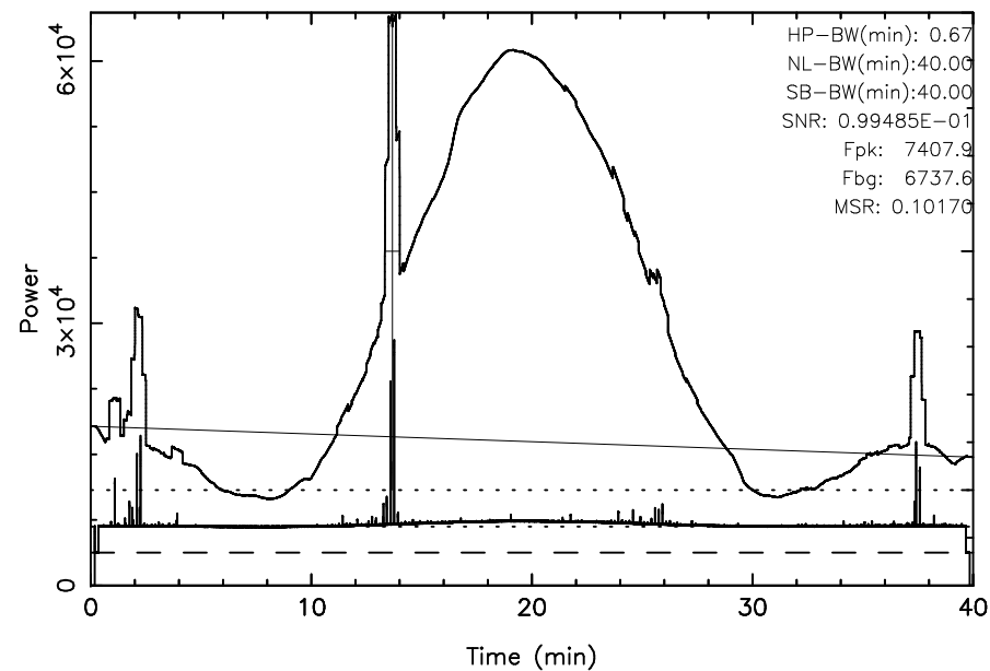
TOYOKAWA 3C10 2024/08/22(235)01:55:15-02:35:15JST
