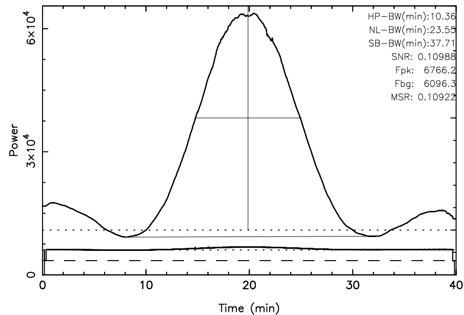
TOYOKAWA 3C10 2024/08/29(242)01:27:44-02:07:44JST
