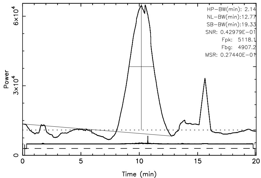
FUJI 3C123 2024/09/05(249)05:21:20-05:41:21JST
