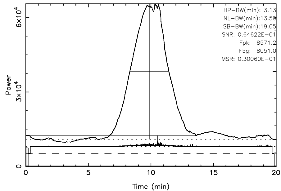
KISO 3C123 2024/09/05(249)05:21:20-05:41:21JST
