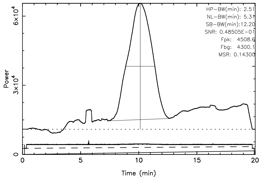
FUJI 3C123 2024/09/14(258)04:45:57-05:05:58JST
