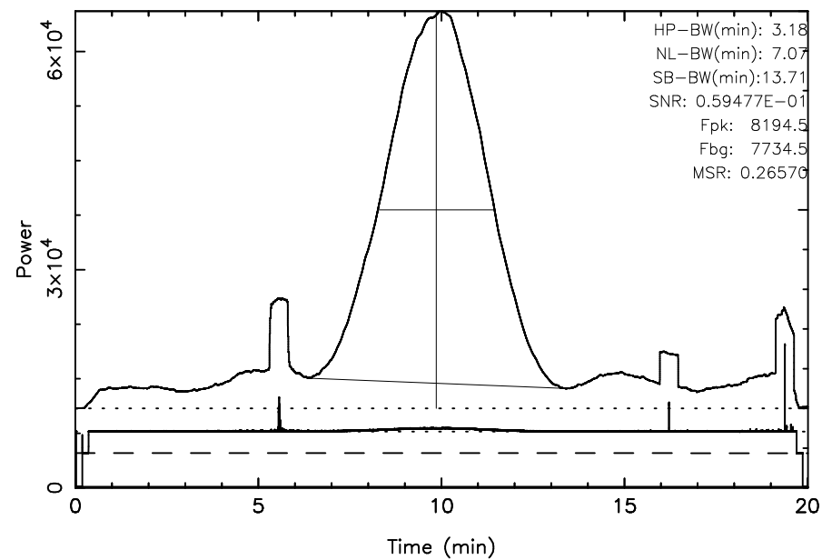
KISO 3C123 2024/09/14(258)04:45:57-05:05:58JST
