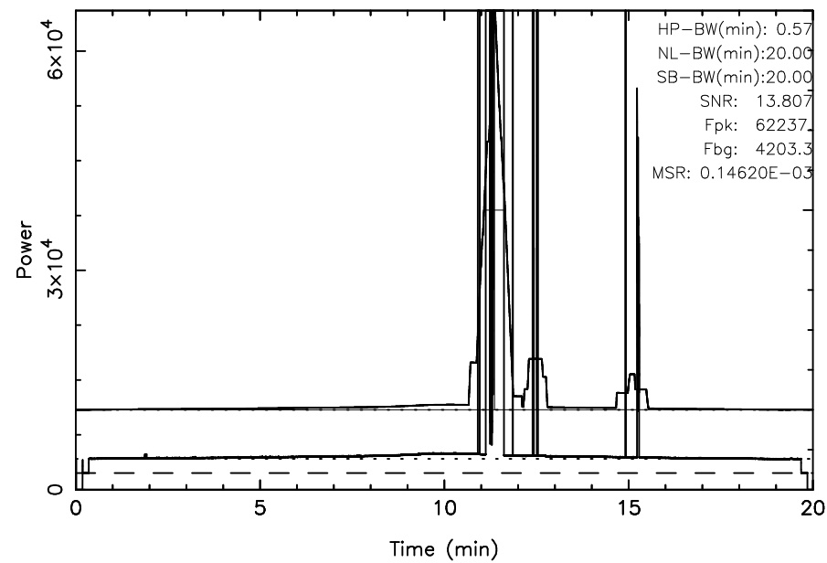
FUJI 3C392 2024/09/16(260)18:54:28-19:14:28JST
