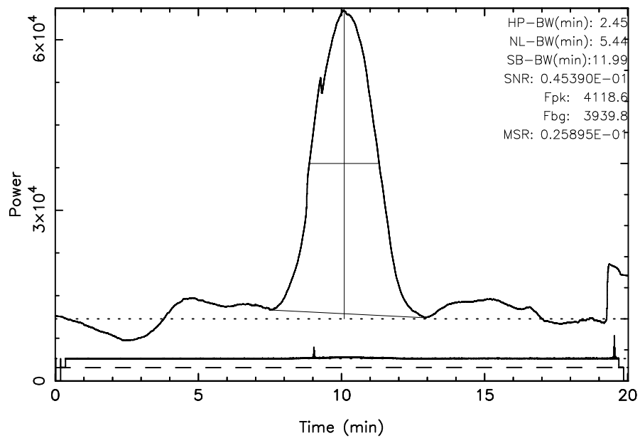
FUJI 3C123 2024/09/16(260)04:38:06-04:58:07JST
