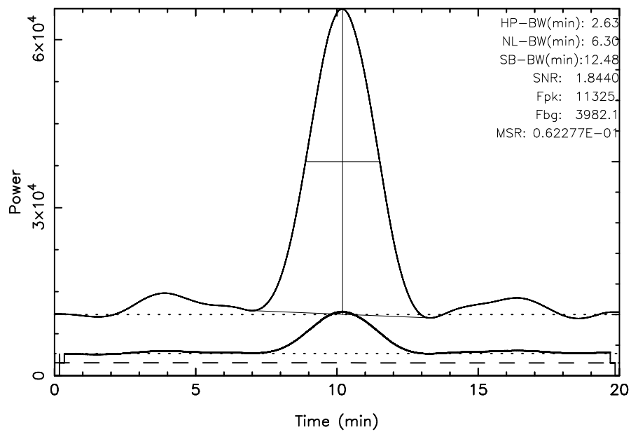
FUJI 3C405 2024/09/16(260)19:57:16-20:17:16JST
