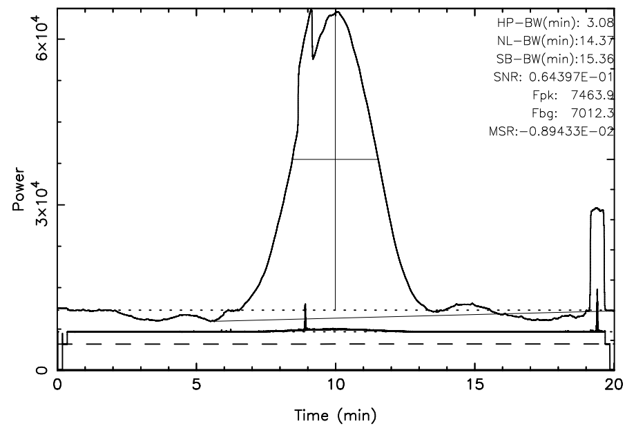
KISO 3C123 2024/09/16(260)04:38:06-04:58:07JST
