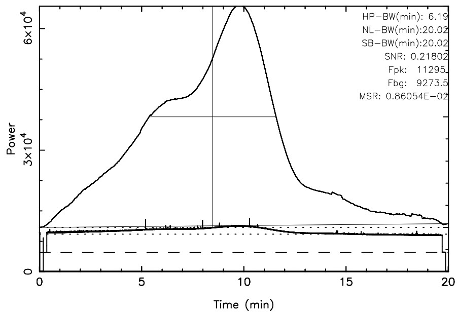
KISO 3C392 2024/09/18(262)18:46:36-19:06:37JST
