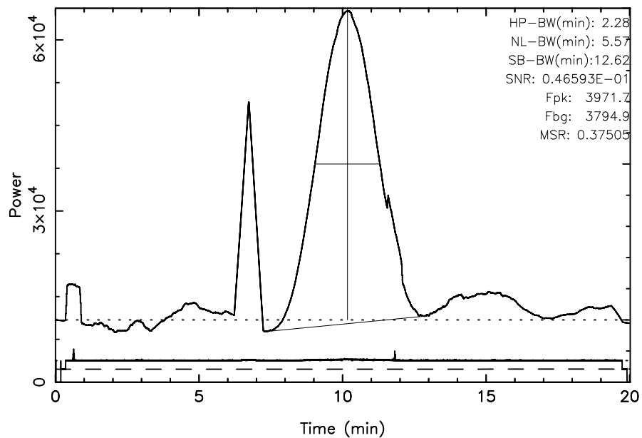
FUJI 3C123 2024/09/18(262)04:30:14-04:50:15JST
