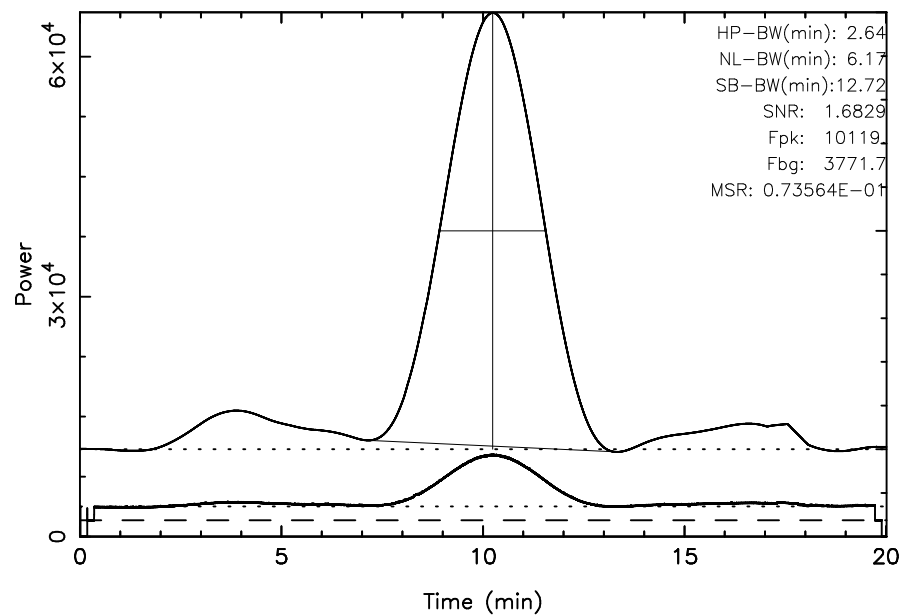
FUJI 3C405 2024/09/18(262)19:49:24-20:09:25JST
