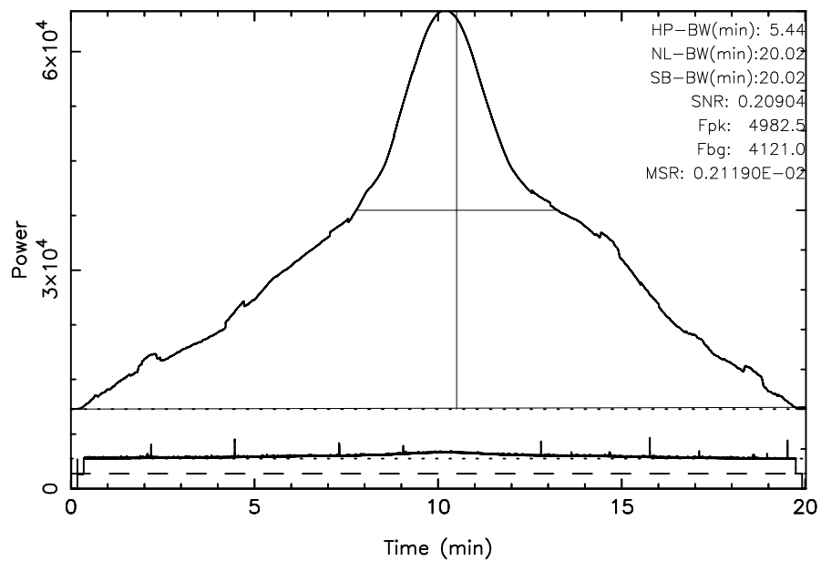
FUJI 3C392 2024/09/18(262)18:46:36-19:06:37JST
