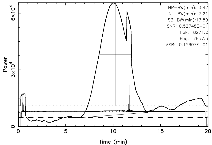
KISO 3C123 2024/09/18(262)04:30:14-04:50:15JST
