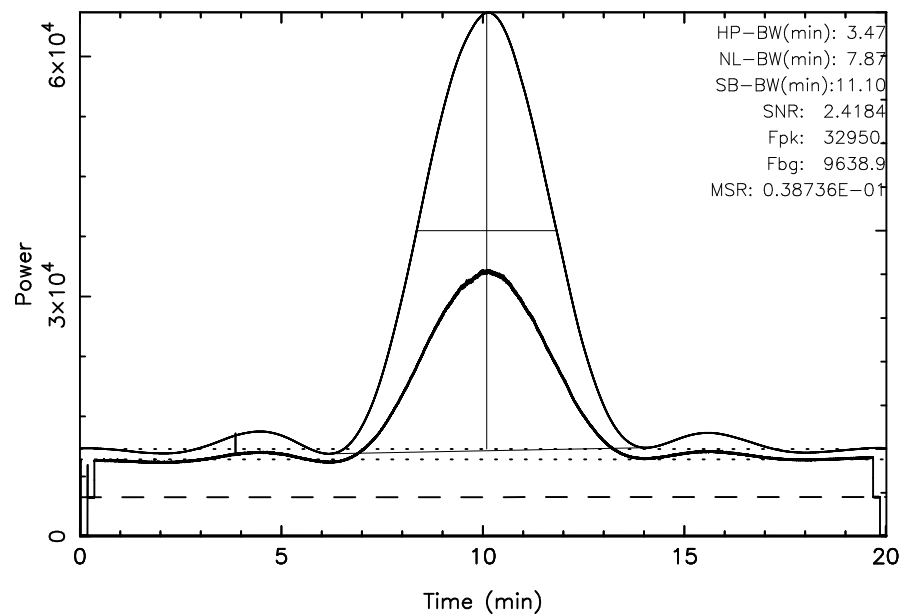
KISO 3C405 2024/09/18(262)19:49:24-20:09:25JST
