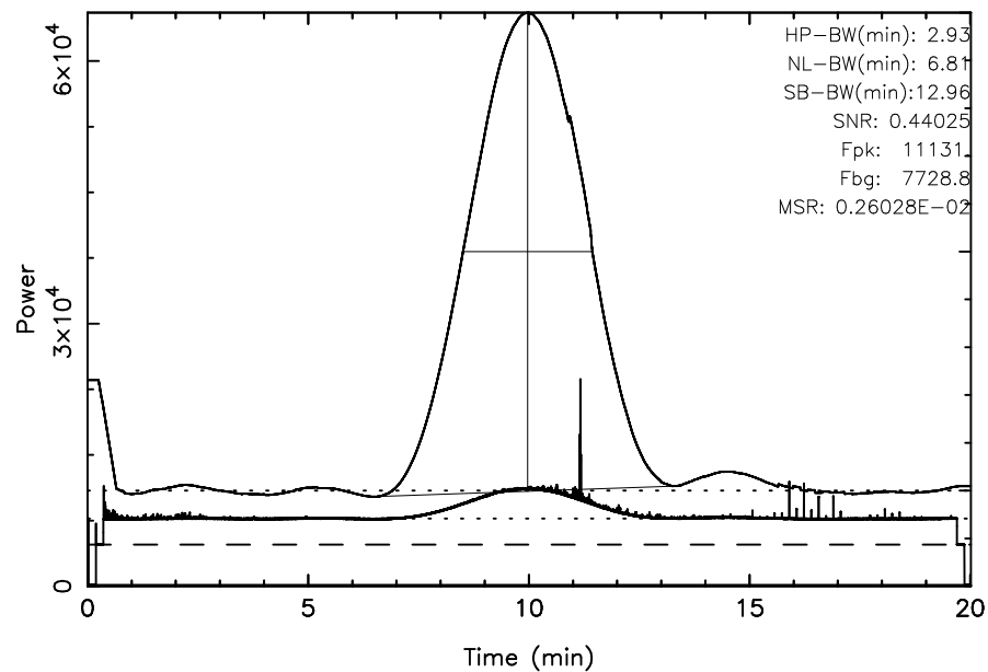
KISO 3C144 2024/09/18(262)05:27:26-05:47:27JST
