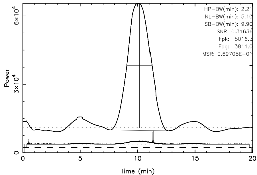
FUJI 3C144 2024/09/18(262)05:27:26-05:47:27JST
