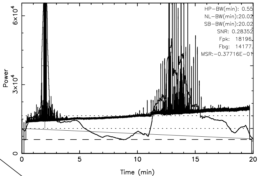
KISO 3C123 2024/09/25(269)04:02:42-04:22:43JST
