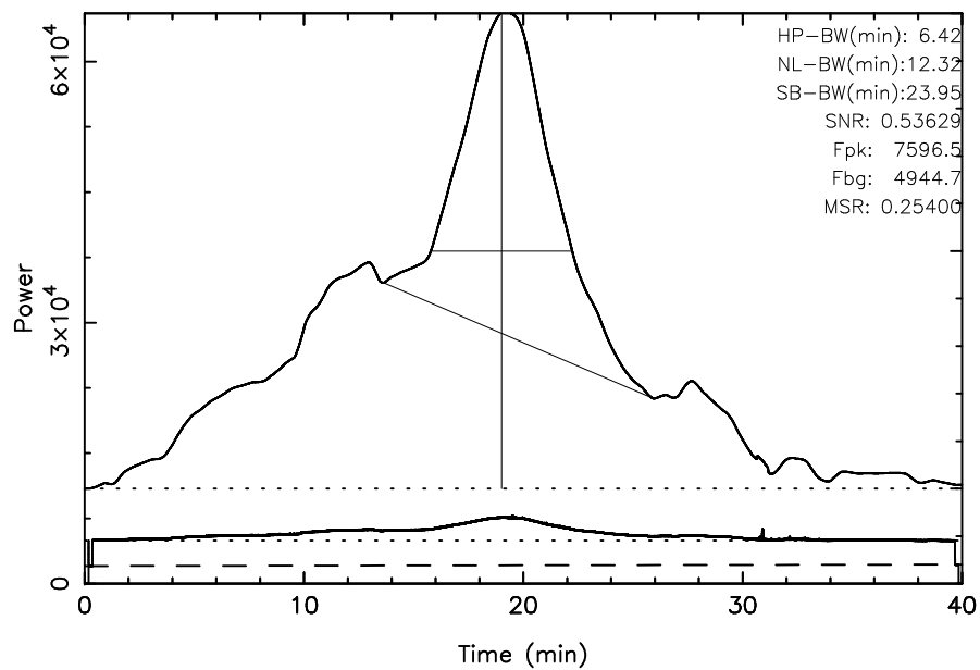
TOYOKAWA 3C392 2024/09/03(247)19:35:35-20:15:35JST
