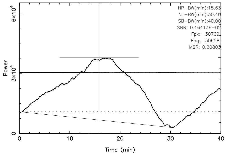
TOYOKAWA 3C461 2024/09/03(247)00:05:56-00:45:56JST
